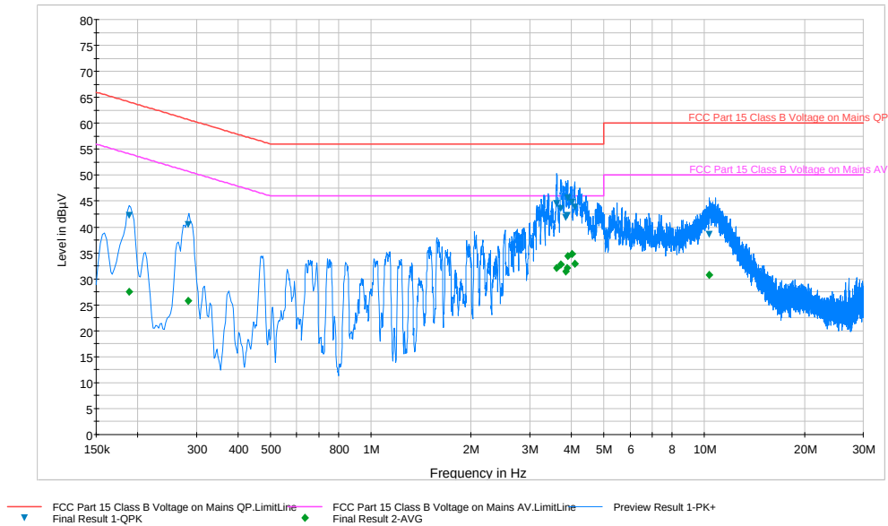
Plot 6-26. Line Conducted Plot with 802.11a UNII Band 1 (N)
