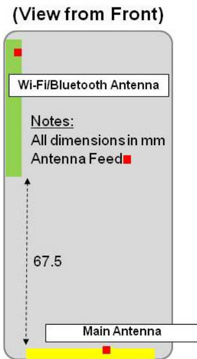
Figure 2: Antenna Separation Distances
