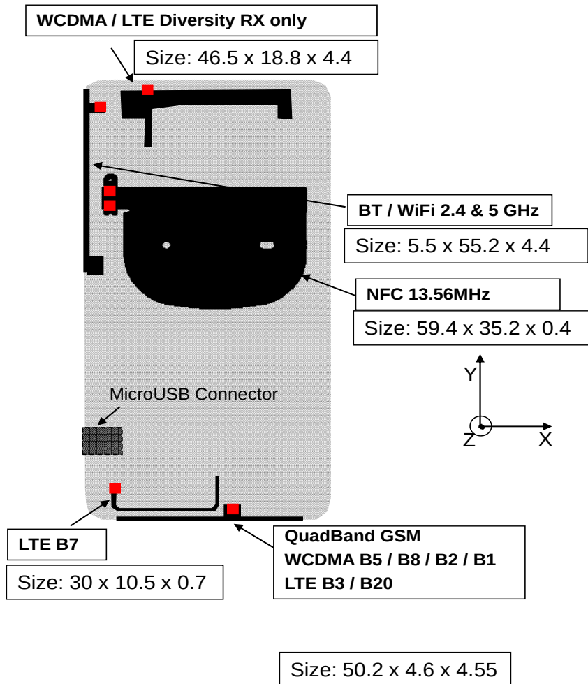
Photograph 9-3: Locations and Spacings of Antennas.
