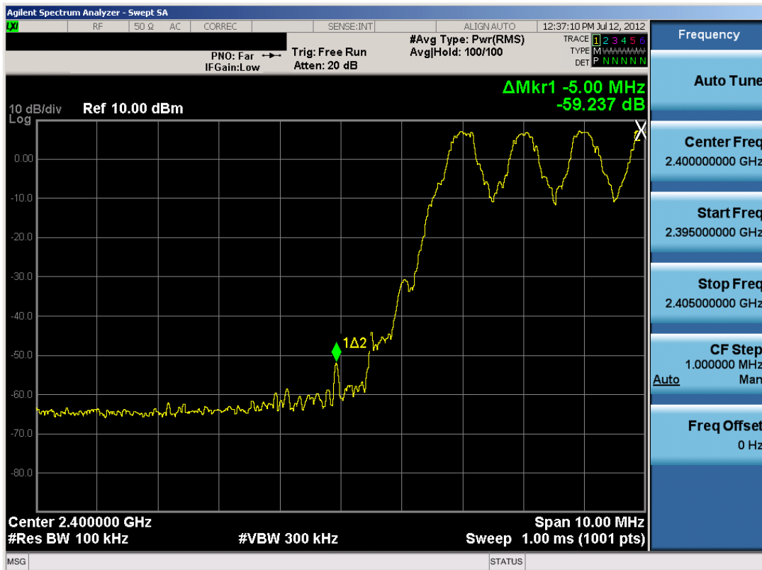
Plot 6-12. Band Edge Plot (Bluetooth with Hopping Enabled, 1Mbps)
