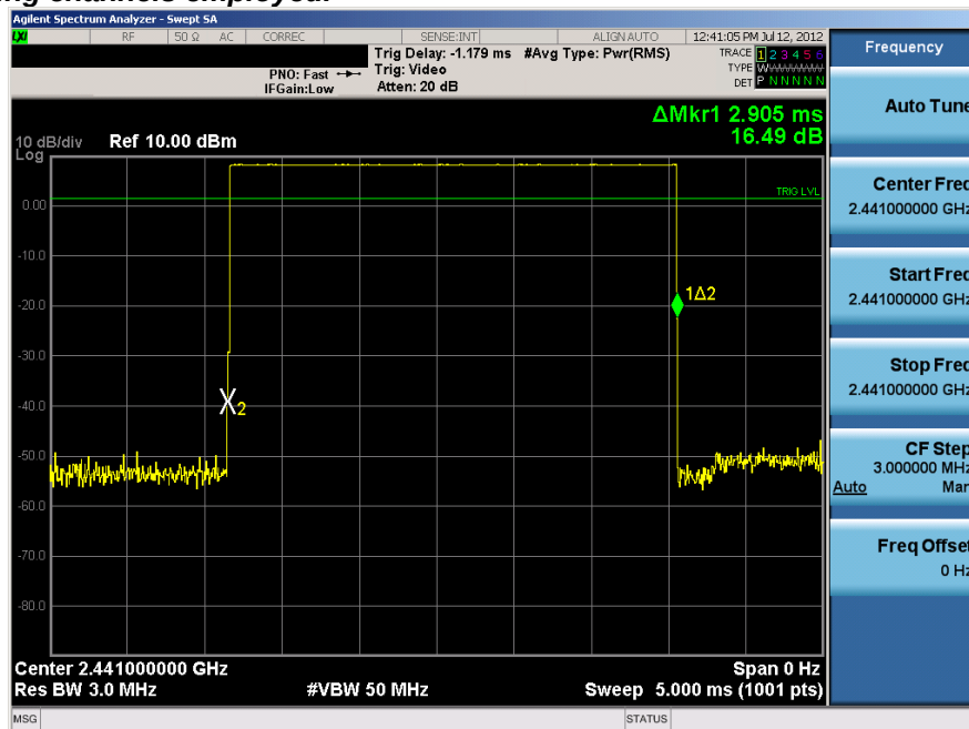
Plot 6-15. Time of Occupancy Plot (Bluetooth)
