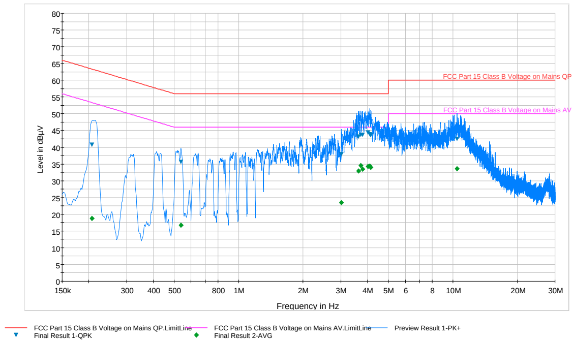
Plot 6-25. Line-Conducted Test Plot (N)
