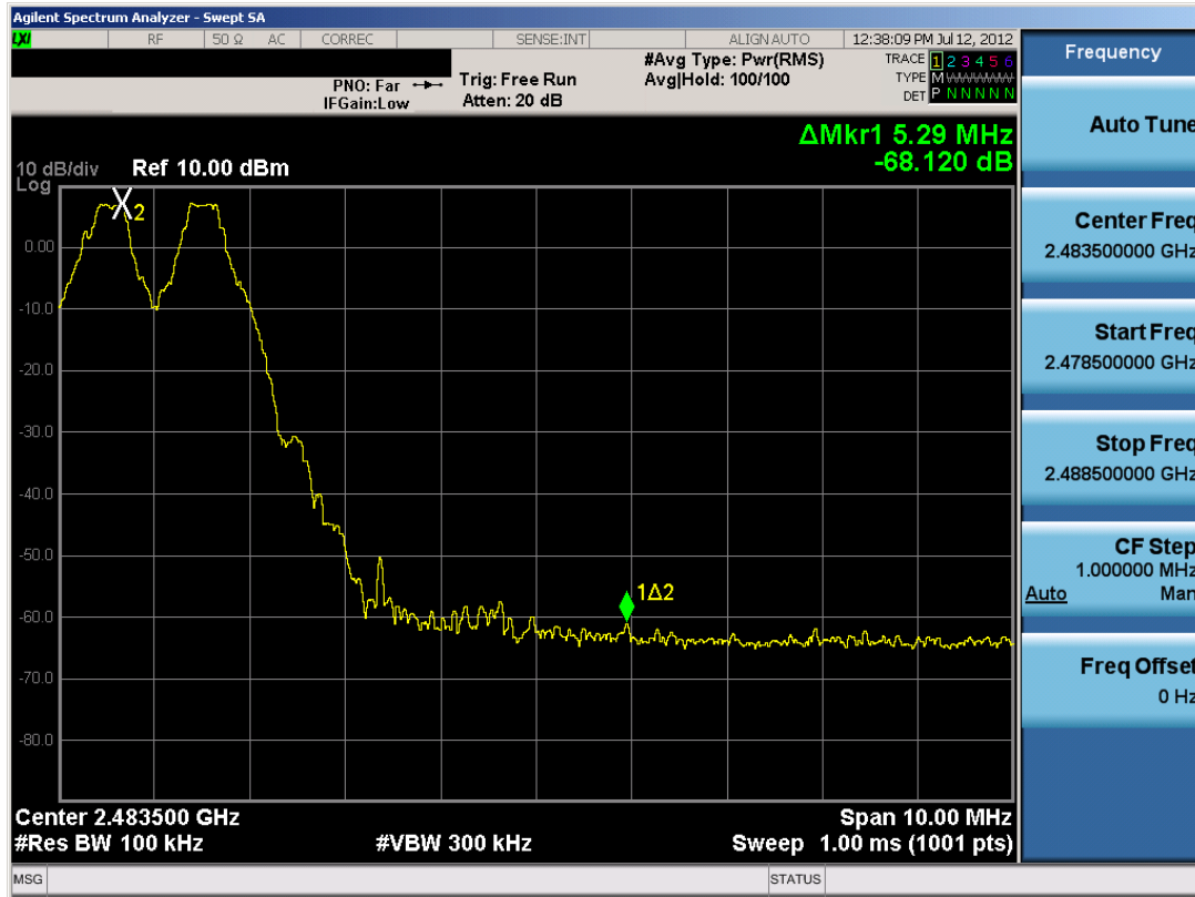
Plot 6-13. Band Edge Plot (Bluetooth with Hopping Enabled, 1Mbps)
