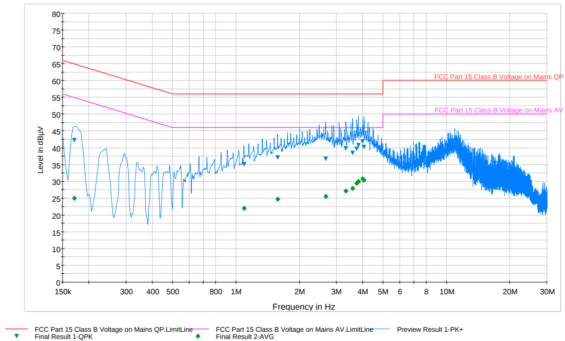
Plot 6-24. Line-Conducted Test Plot (L1)
