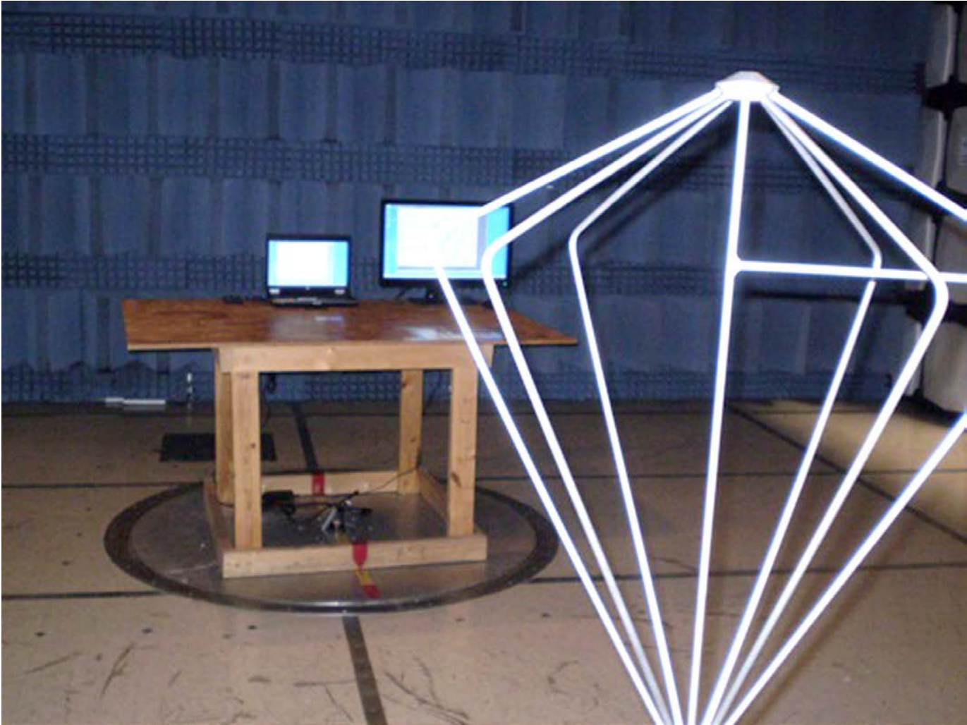
Figure 7c1-2: Part 15B Spurious Radiations Test Configuration.
