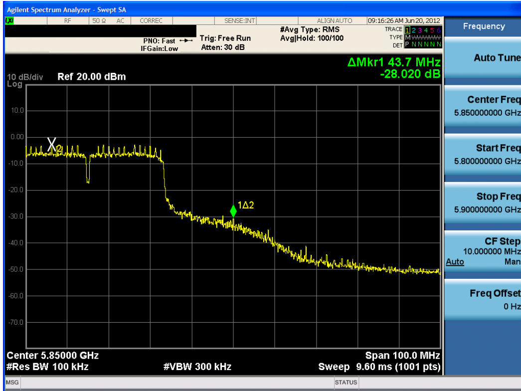
Plot 6-54. Band Edge Plot (40MHz BW 802.11n (5.8GHz) – Ch. 163)
