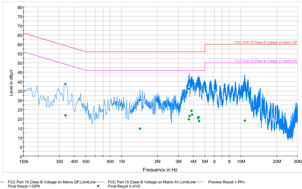
Plot 6-67. Line Conducted Plot with 802.11b (L1)
