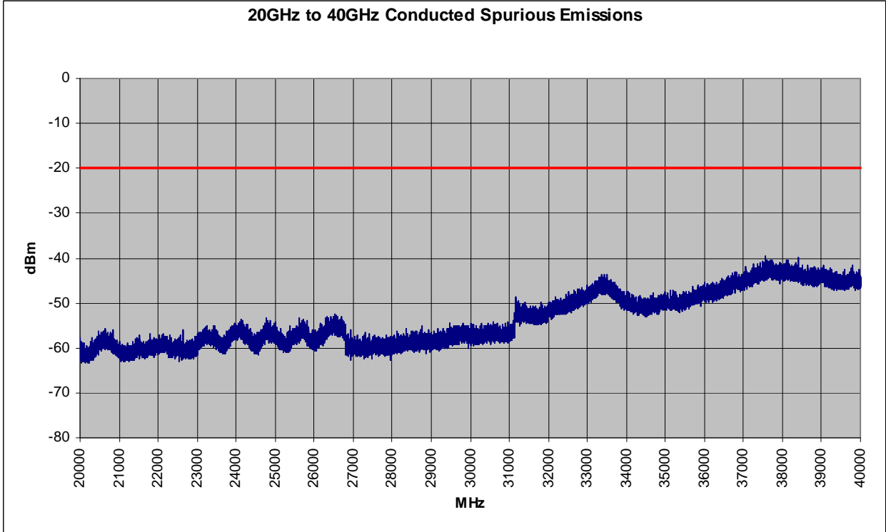
Plot 6-64. Conducted Spurious Plot (802.11a – Ch. 157)
