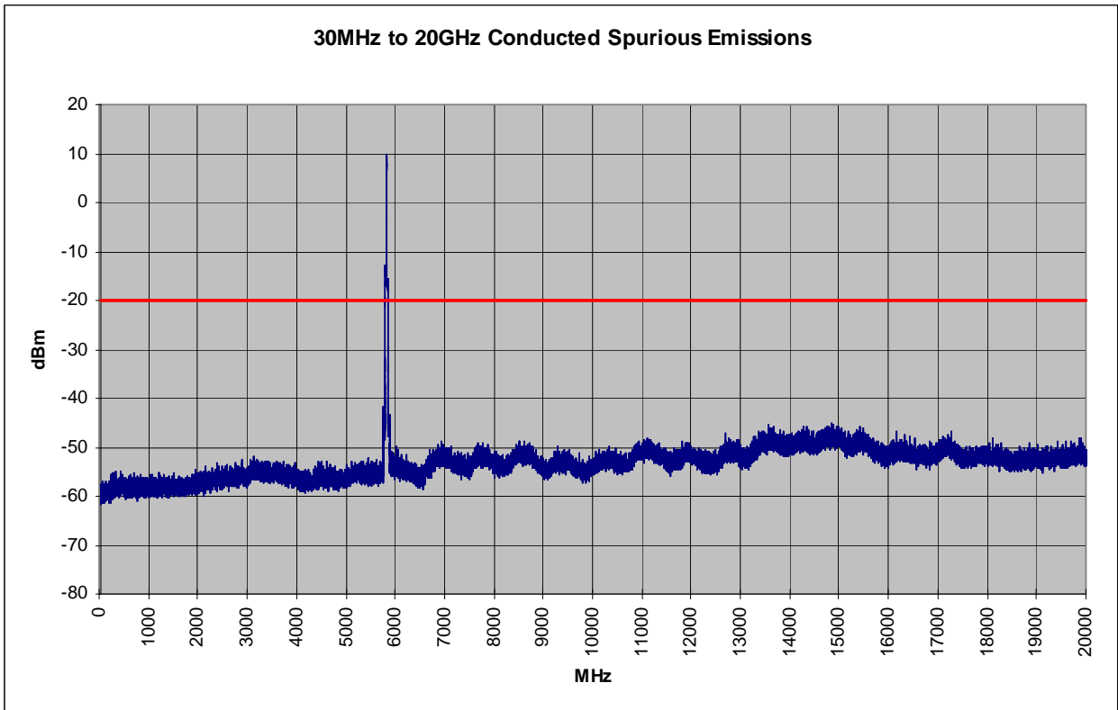
Plot 6-65. Conducted Spurious Plot (802.11a – Ch. 165)
