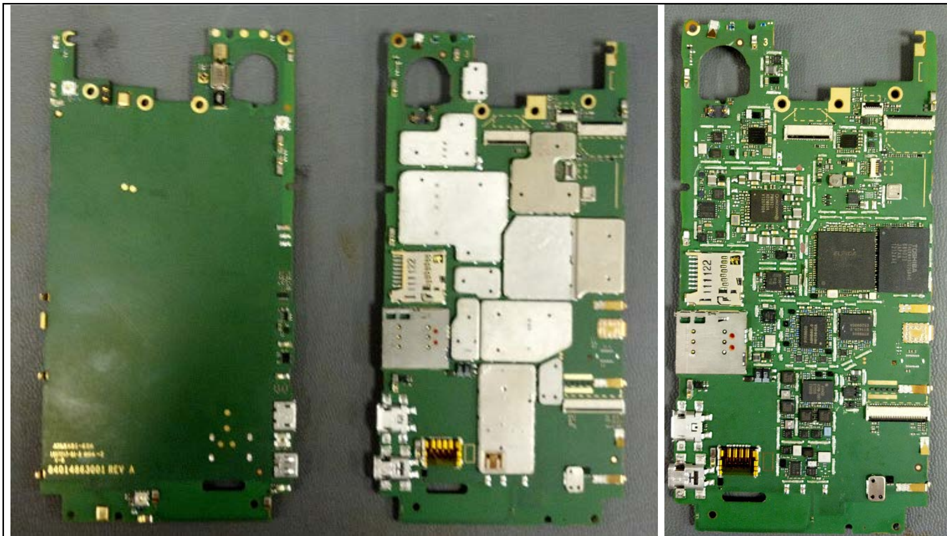
Photograph 9-2: Main PC Board, Shown with and without Shields in place (Component Side) and Non-Component Side.
