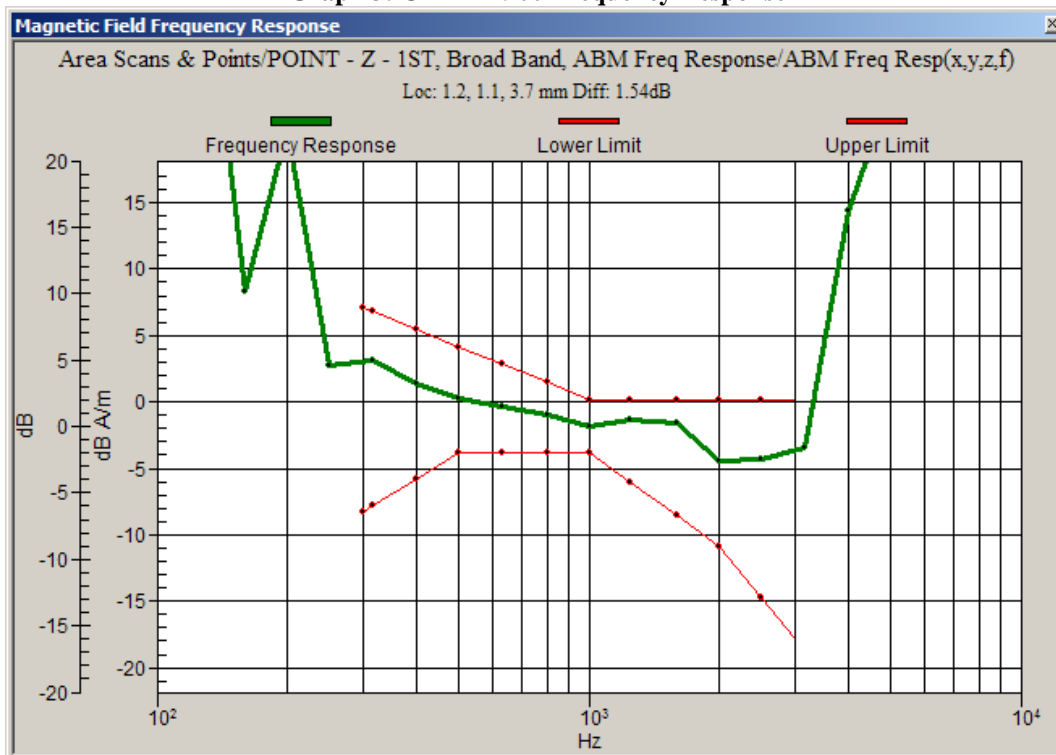
Graph 3: CDMA 1900 Frequency Response
