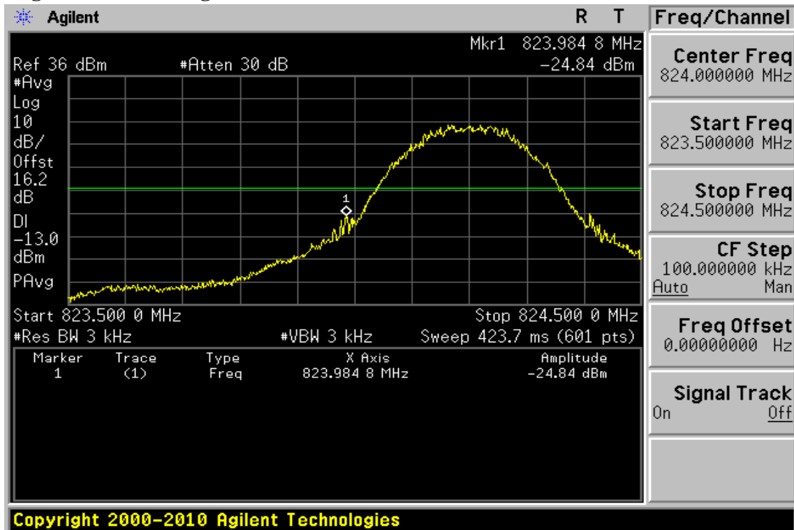
Figure 9-24: Bad edge emission at antenna terminals –EDGE 850 Channel Lowest
