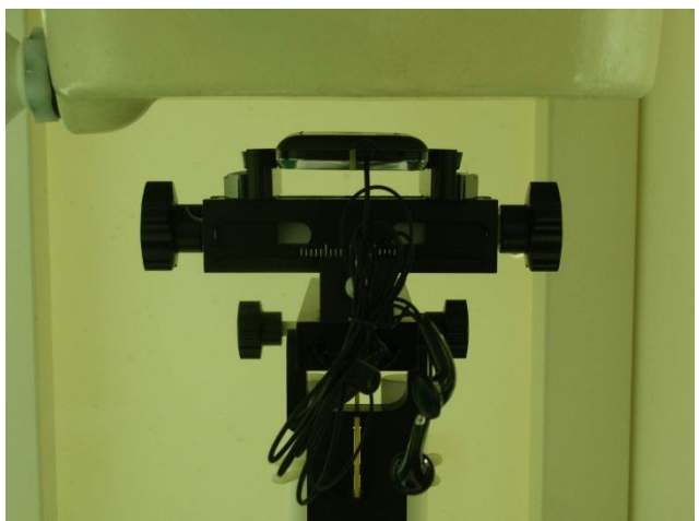
Back of the DUT with Phantom 1.5 cm Gap (DUT with Earphone)
