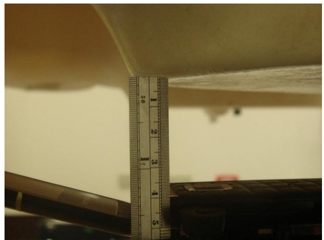
Right Cheek position - Separation distance 4cm between mouth and antenna
