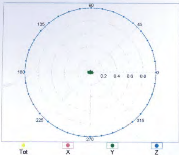
f=600 MHz, TEM, 90^\circ
