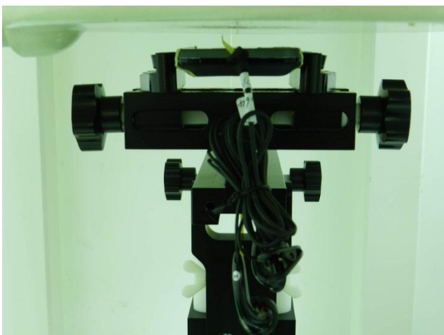
Front of the DUT with Phantom 1 cm Gap (Headset)
