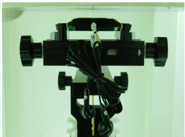
Back of the DUT with Phantom 1 cm Gap (Headset)
