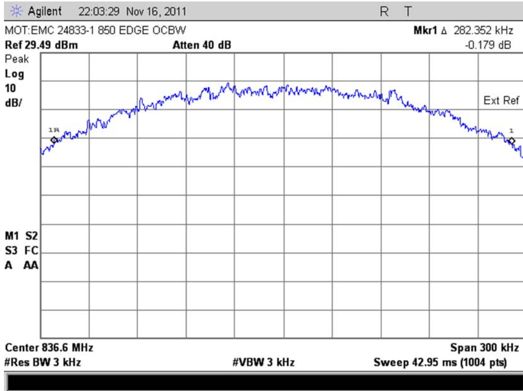
EDGE 850 – Channel 190 (836.60 MHz) – Occupied Bandwidth
