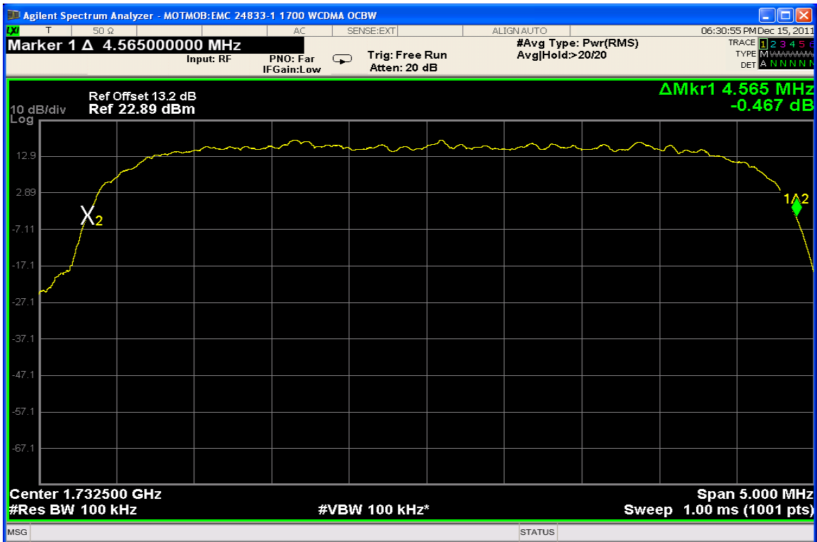
WCDMA 1700 – Occupied Bandwidth – Channel 1413 (1732.5 MHz)
