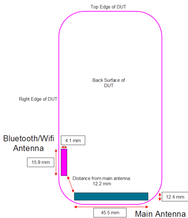
Figure 2: Antenna Separation Distances
