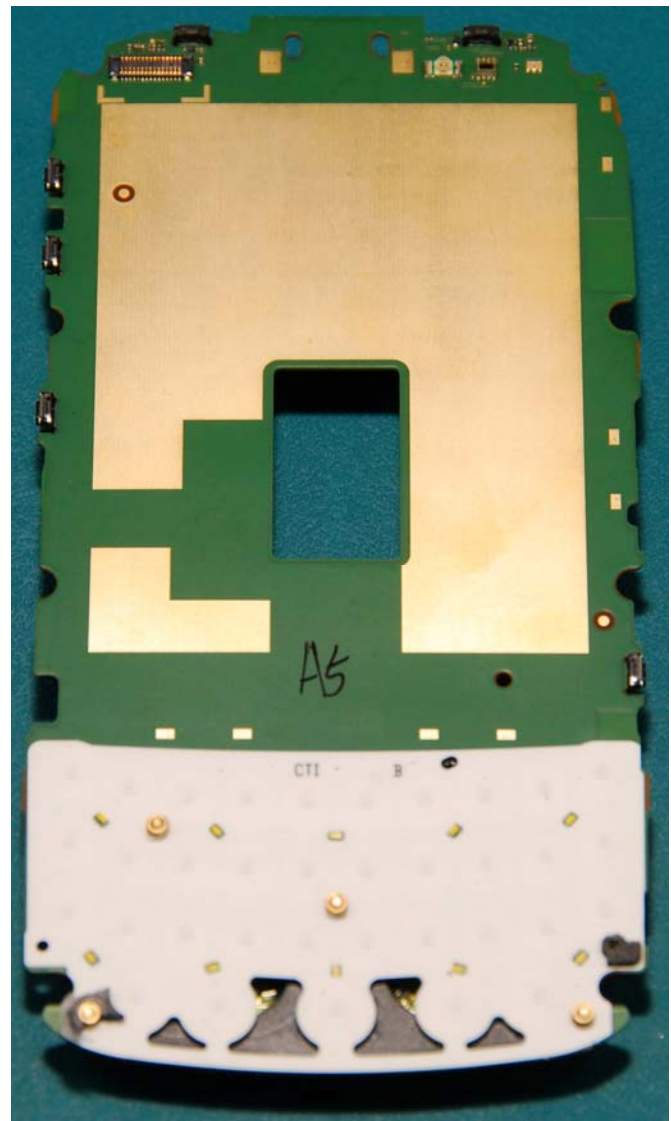
Keypad Board
