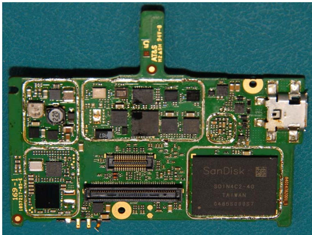
Main Board-Bottom (Shielding removed)
