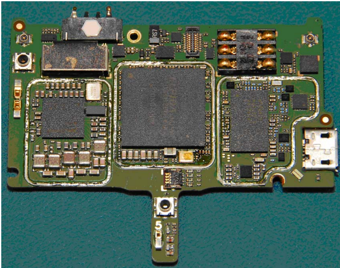
Main Board-Top (Shielding removed)
