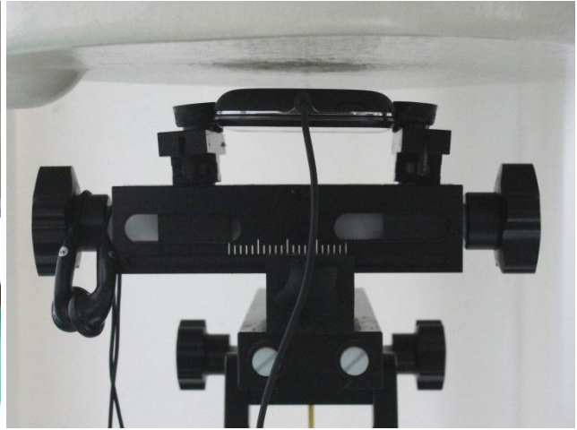
Rear Face of the DUT with Phantom 1 Gap (DUT with Earphone)
