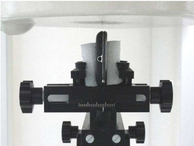
Right Side of the DUT Phantom 1 cm Gap
