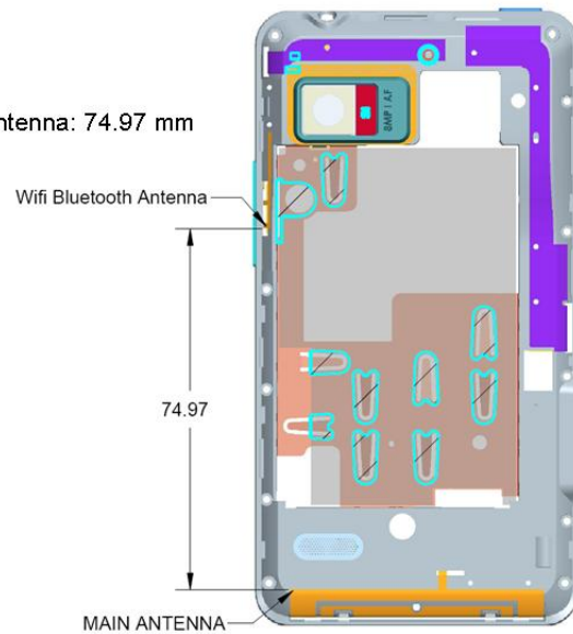
Figure 2: Antenna Separation Distances
