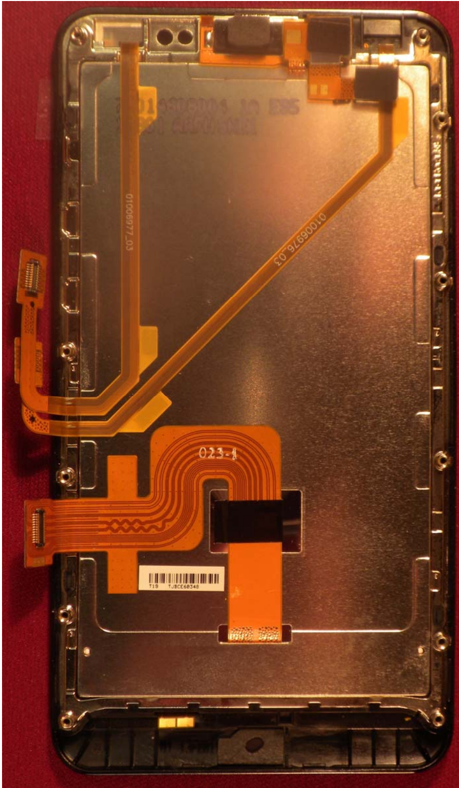
Back up display with Flex
