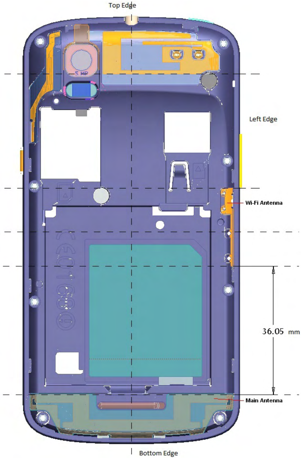
Figure 2: Antenna Separation
