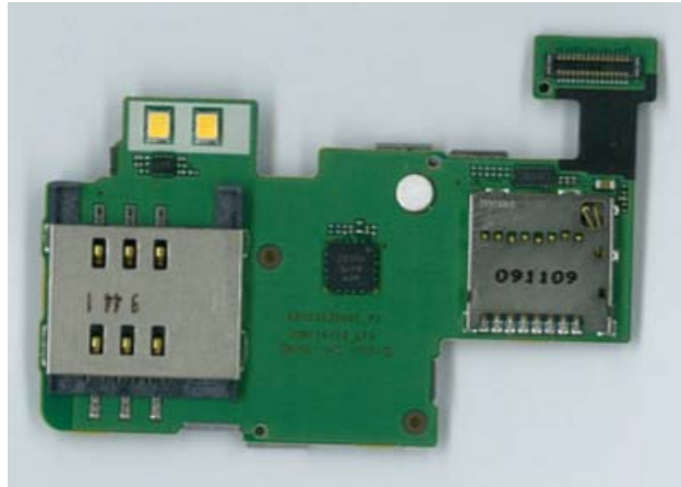
Daughter Board Top
