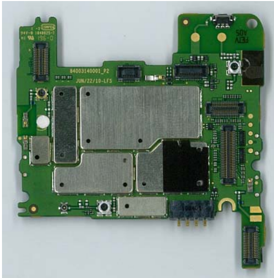
Main Board Top With shields
