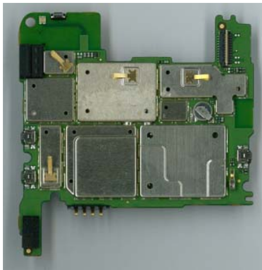
Main Board Bottom With Shields
