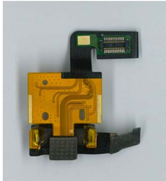
Headset Jack Flex Bottom
