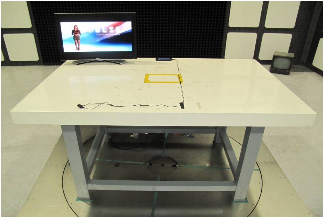
Radiated Emission Test Setup Photo (config 4)
