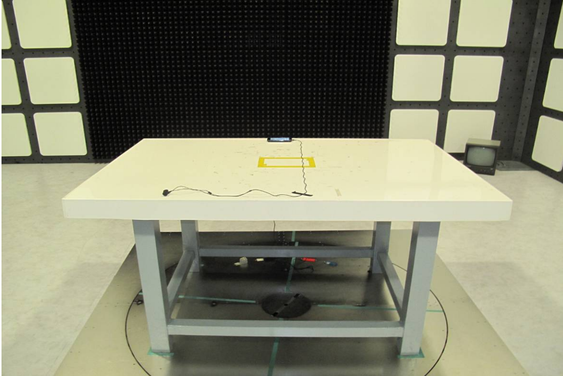
Radiated Emission Test Setup Photo (config 1, 2, 5, 7)
