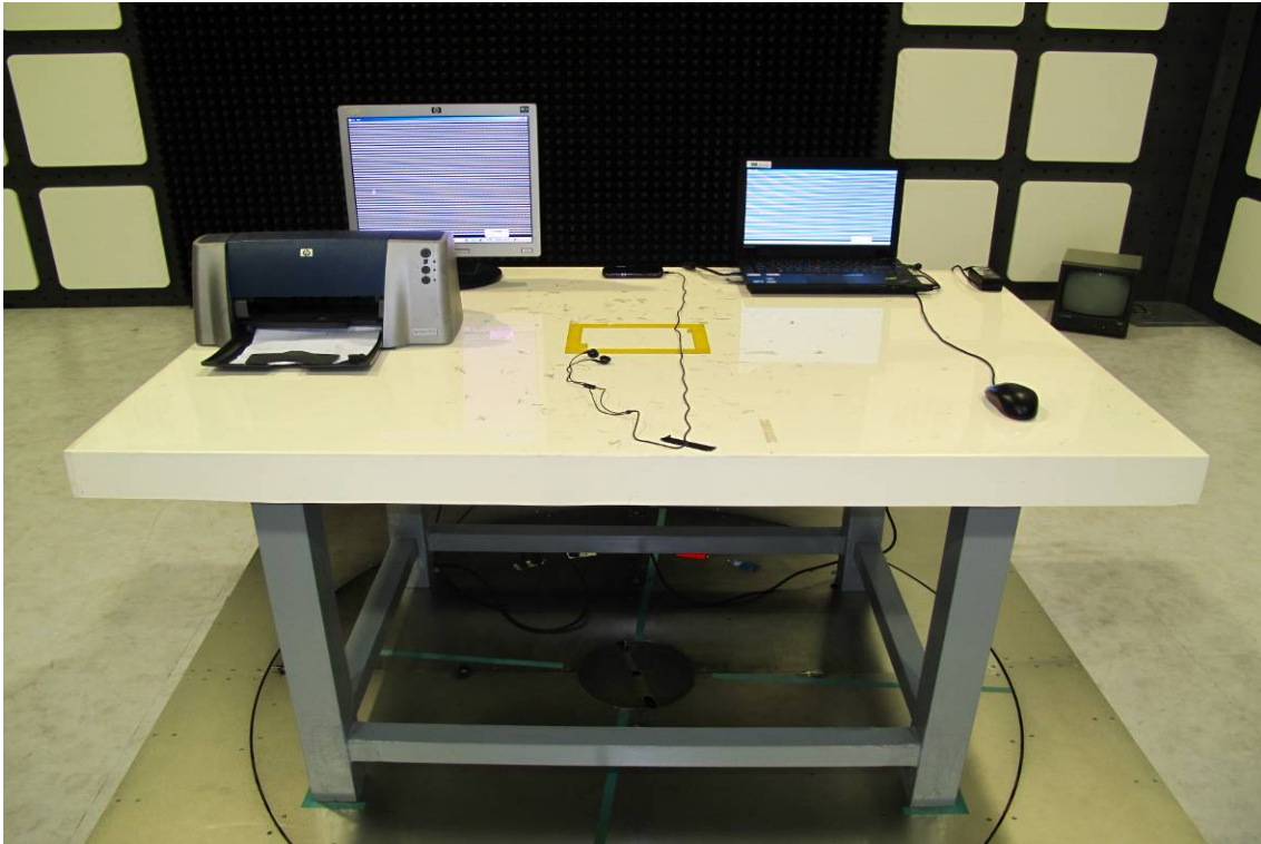
Radiated Emission Test Setup Photo (config 6)
