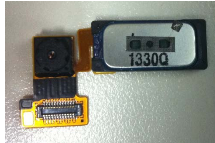
BACK OF ASSY VGA-EARPIECE FLEX
