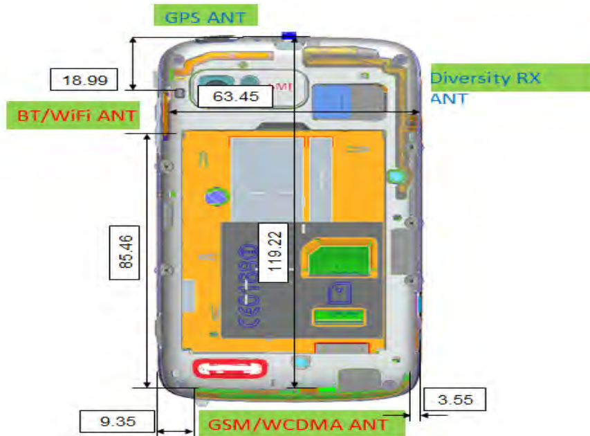
Fig.8 Antenna position of EUT
