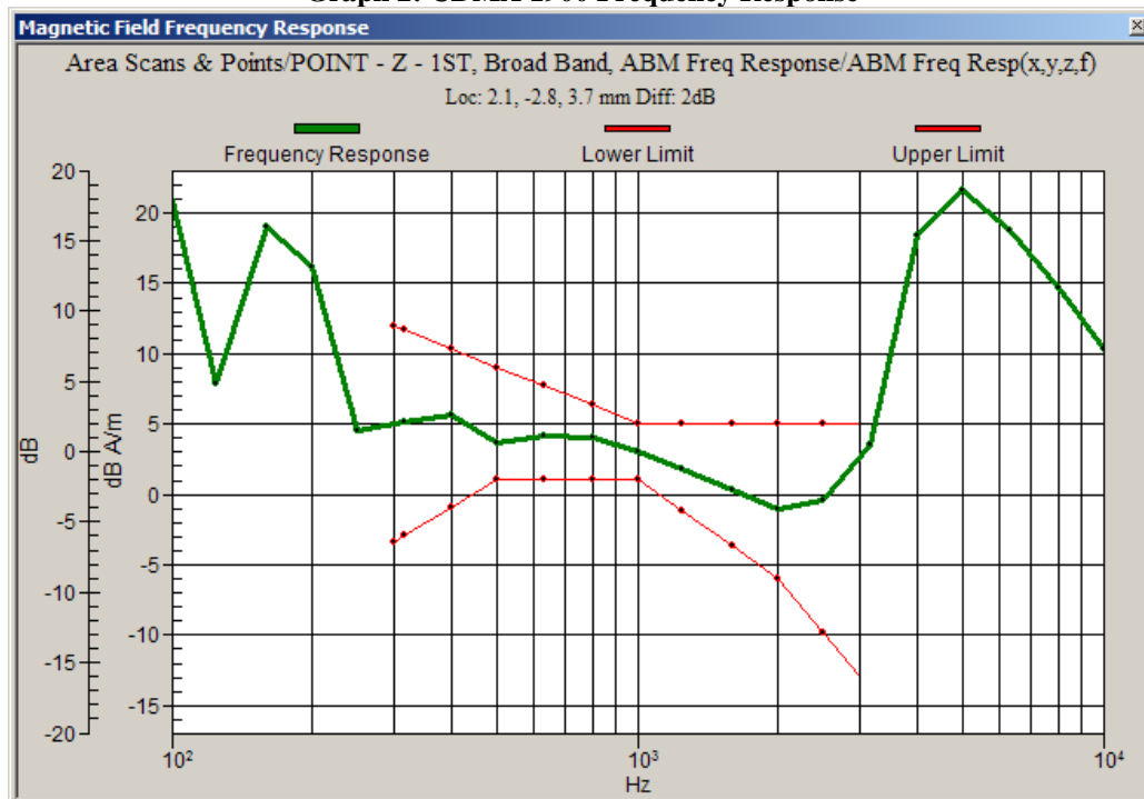
Graph 2: CDMA 1900 Frequency Response
