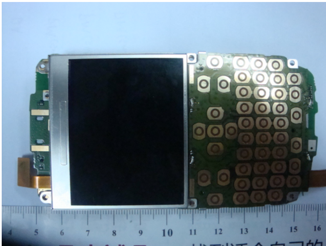
Photograph 9-1: Front side view of radio product PC Board with Keypad PC Board detached.
