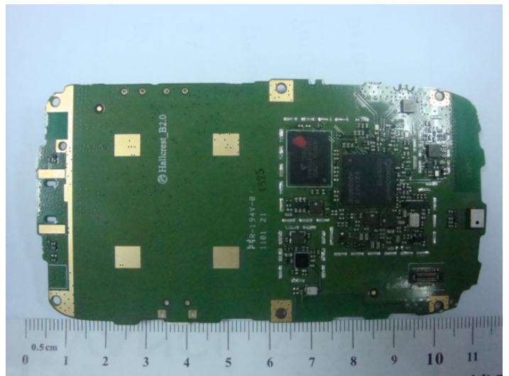
Photograph 9-3: Front and Back side view of radio PC Board, without shields.
