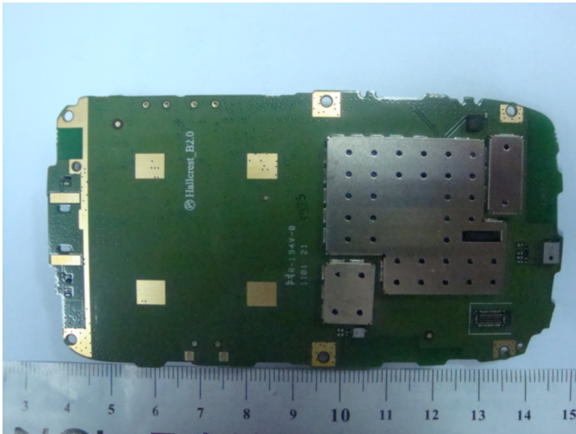
Photograph 9-2: Back side view of radio product Keypad PC Board.
