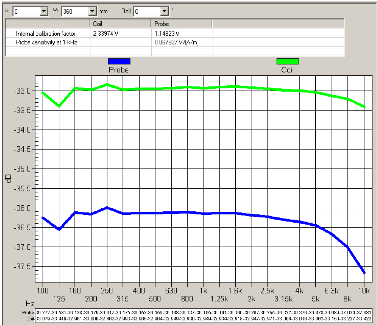
Graph 1: Frequency Response measured in AMCC
