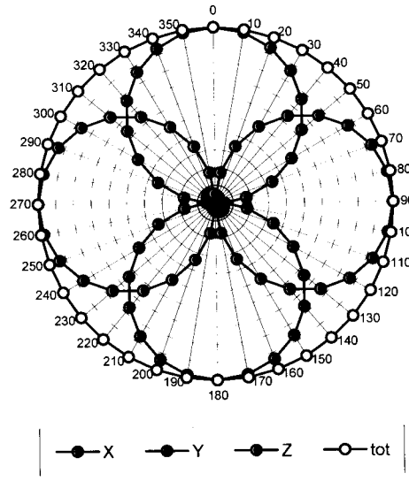
f = 2500 MHz, WG R22
