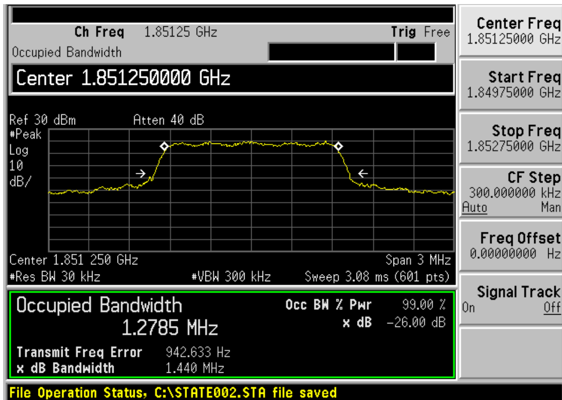
CDMA PCS CH25 Occupied Bandwidth
