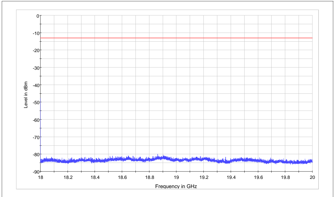
CDMA PCS Channel 25 18GHz ~20GHz
