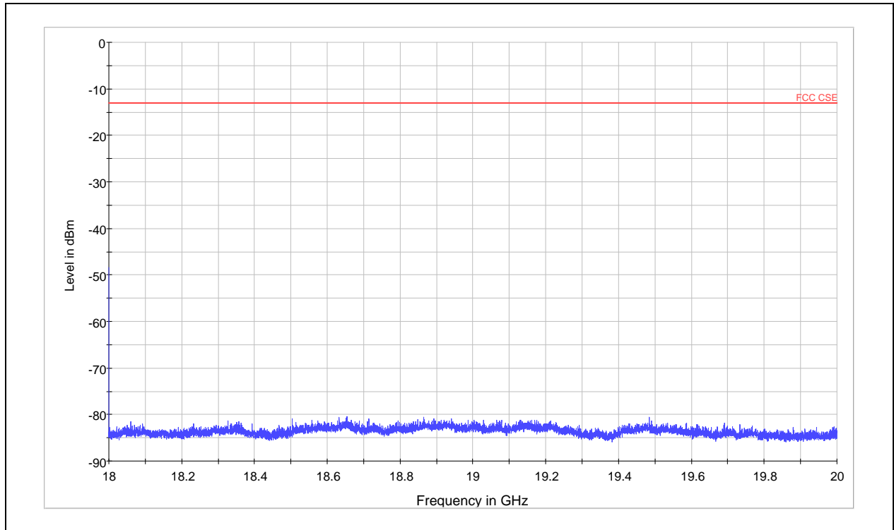
CDMA PCS Channel 600 18GHz ~20GHz
