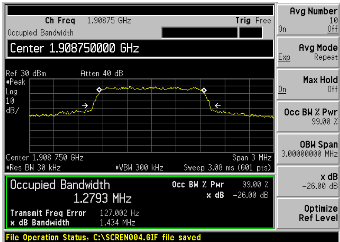
CDMA PCS CH1175 Occupied Bandwidth
