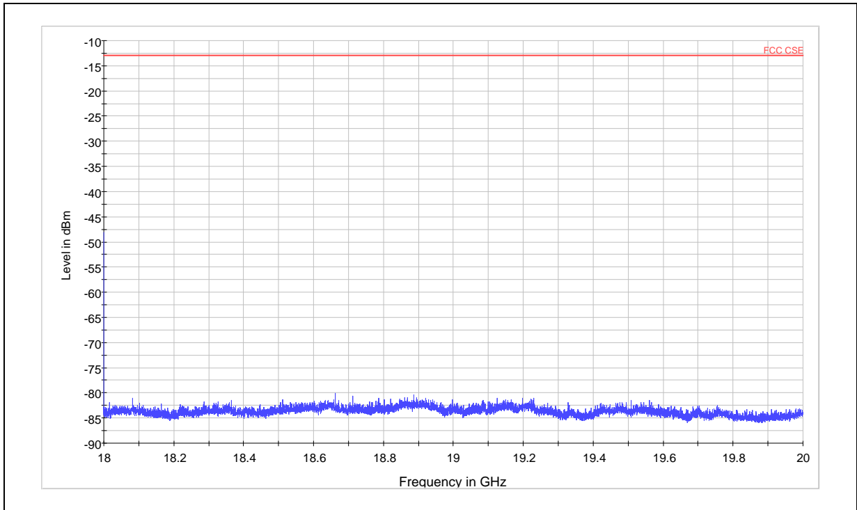
CDMA PCS Channel 1175 18GHz ~20GHz
