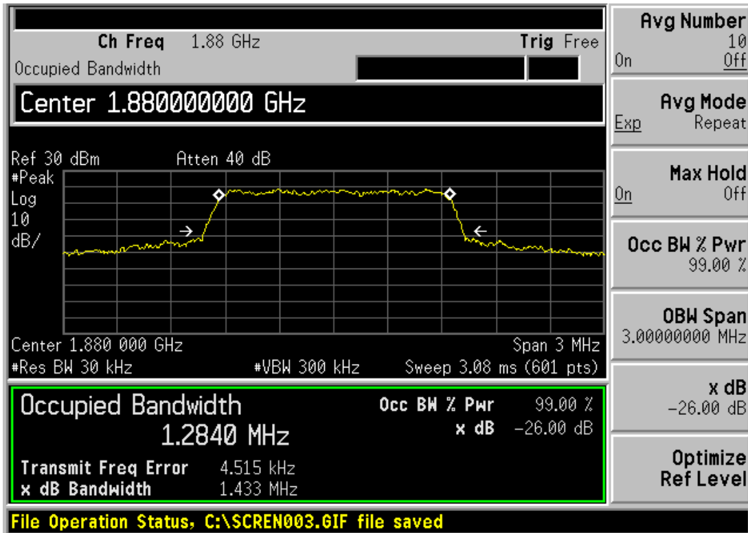
CDMA PCS CH600 Occupied Bandwidth
