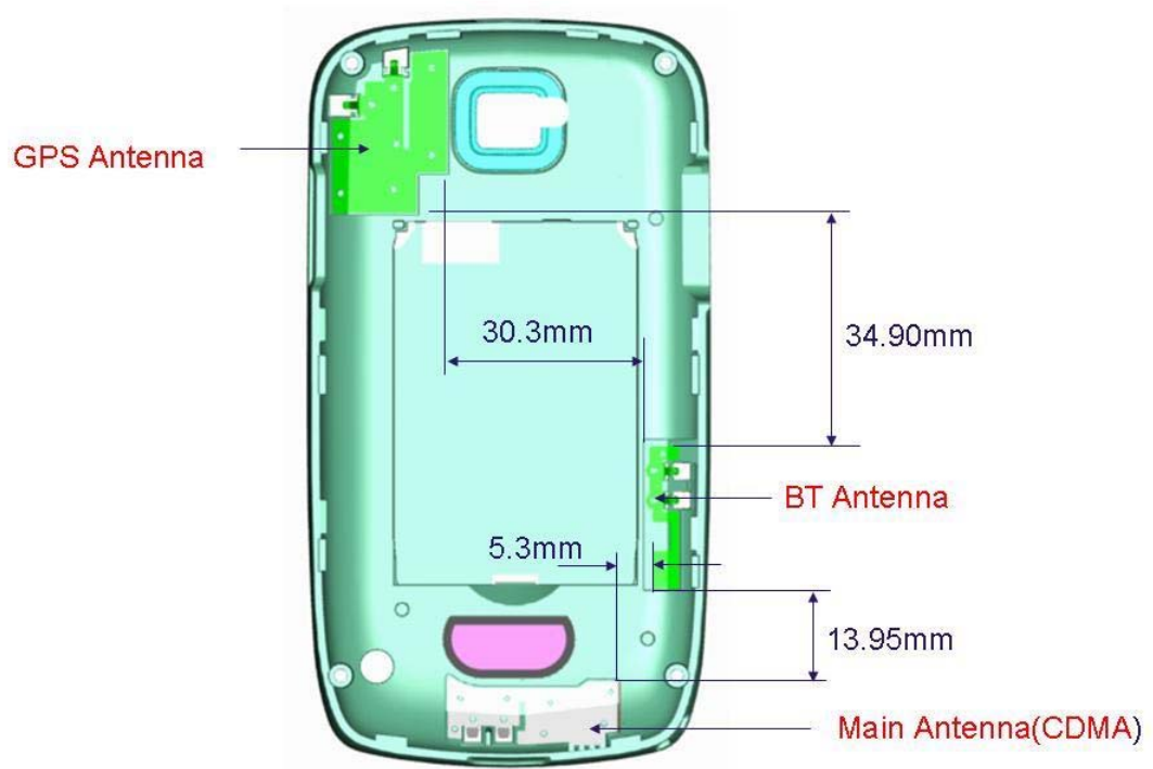
Figure 2: Antenna Separation
