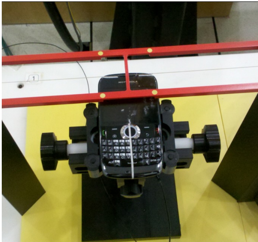
Figure 4. Positioning and Measurement for T-coil
