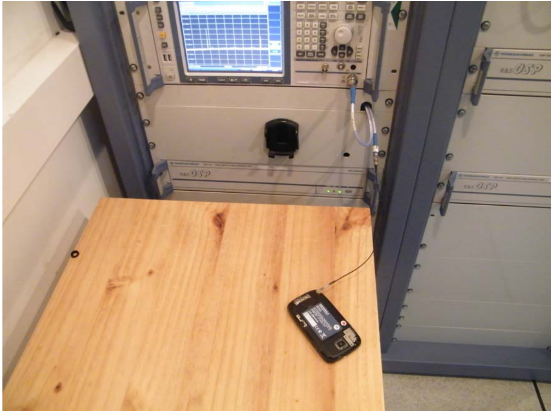
Picture 1: Spurious Emissions at Antenna Terminals Test setup
