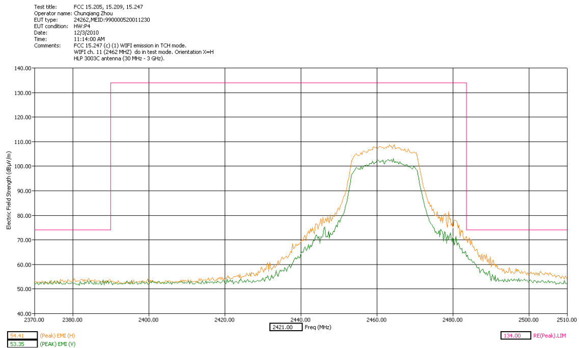
High Band Edge X Orientation Peak Detector
