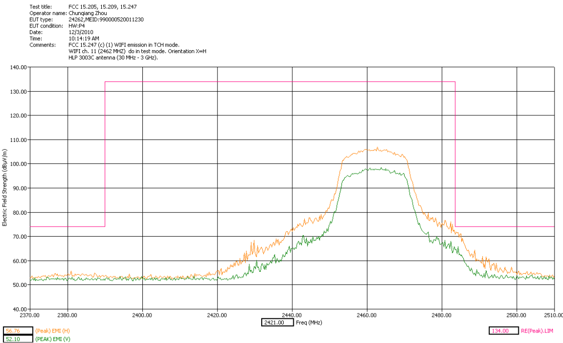
High Band Edge X Orientation Peak Detector
