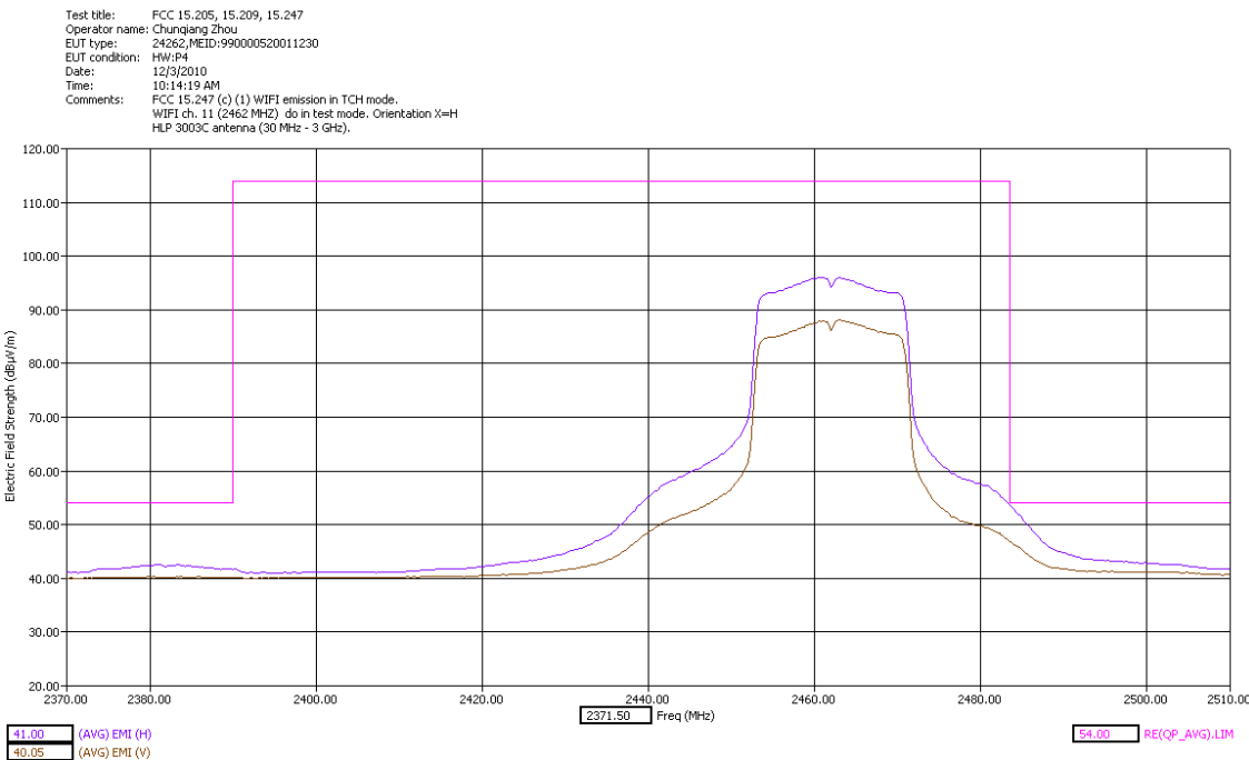
High Band Edge X Orientation AVG Detector
