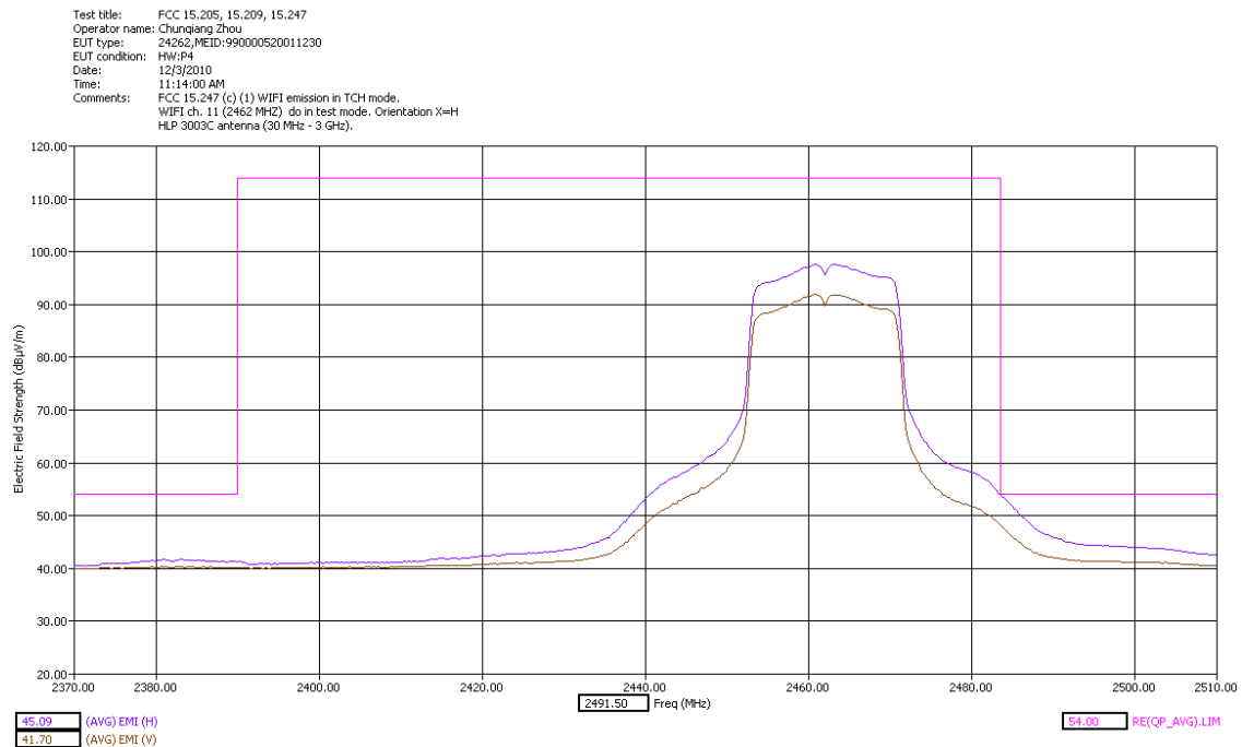
High Band Edge X Orientation AVG Detector
