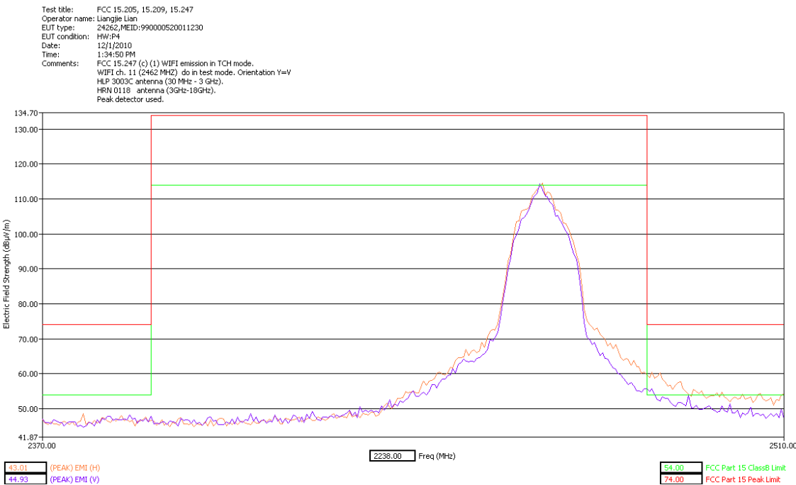
High Band Edge Y Orientation Peak Detector
