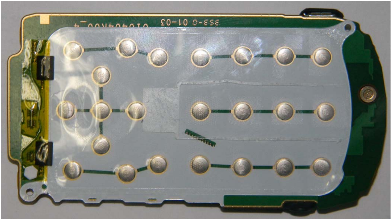
Photograph 9-3: Front side view of radio PC Board, Keypad Popples in Place.
