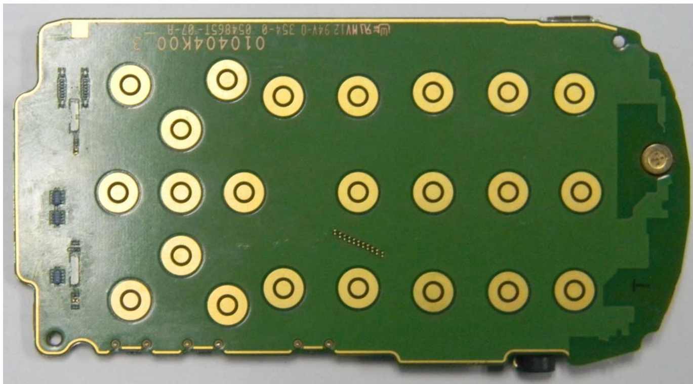
Photograph 9-4: Front side view of radio PC Board, Showing Keypad Base.
