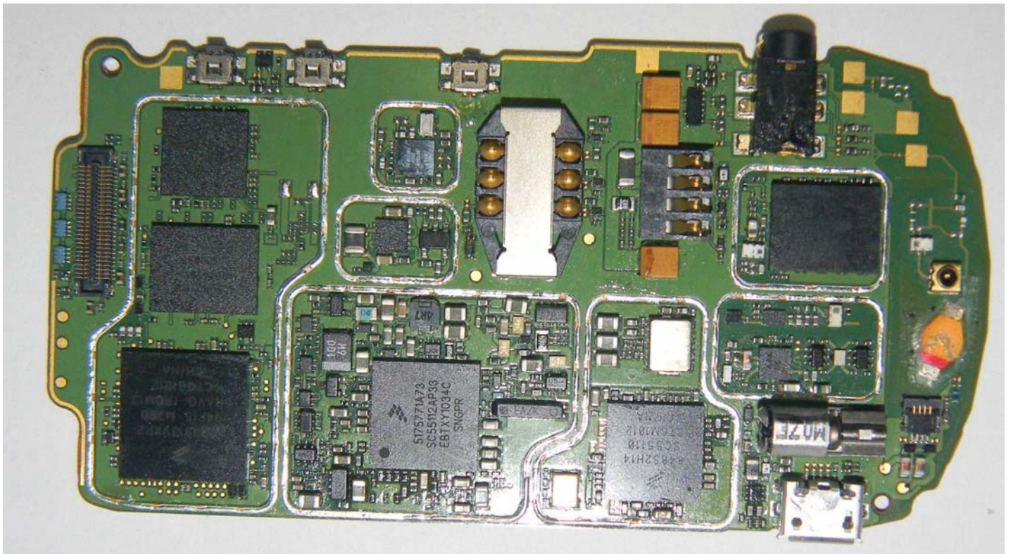
Photograph 9-2: Back side view of radio product PC Board, Shields removed.
