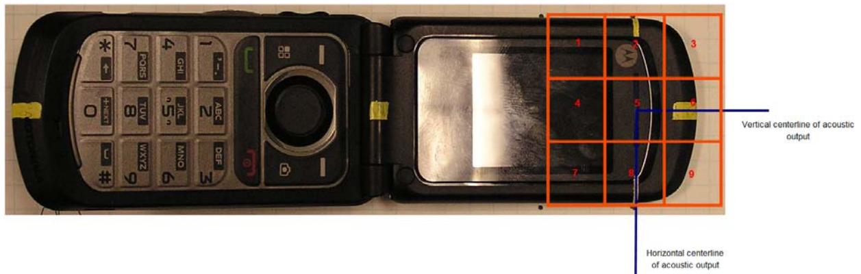
Figure 2. Phone Front - Orientation and Measurement Plane for RF Emissions Testing
