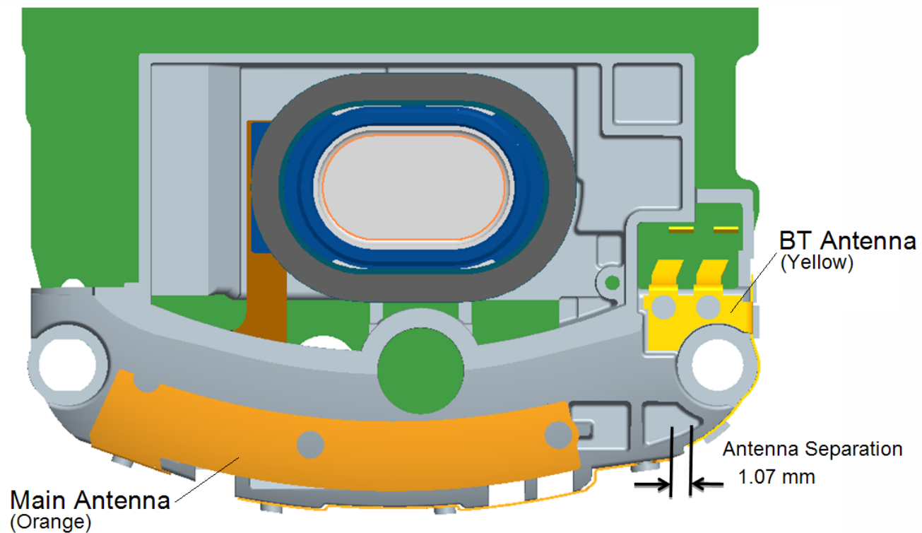
Figure 3: Antenna Separation Distances
