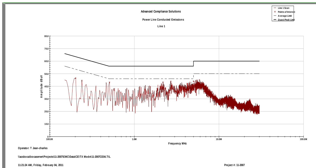
Figure 7.2.2-1: Conducted Emission Line 1
