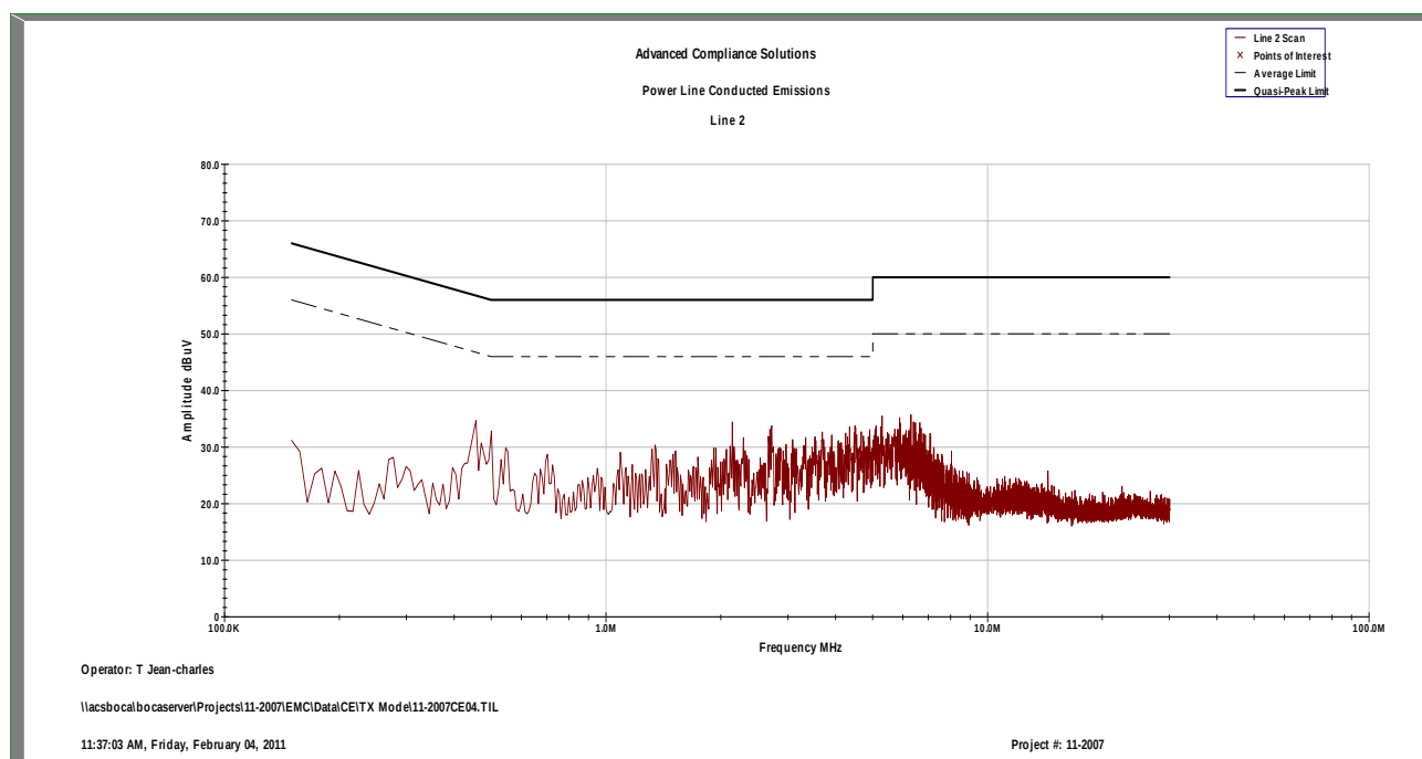
Figure 7.2.2-2: Conducted Emission Line 2
