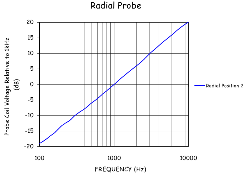
Figure 6-1-3 - Radial Probe sensitivity at 1000 Hz: -60.2 dB V/(A/m)
