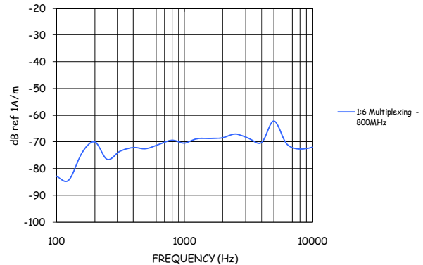
Figure 9-2-2: 800 MHz Undesired Signal (1:6).
