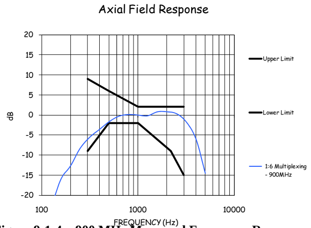
Figure 9-1-4: 900 MHz Measured Frequency Response (1:6).
