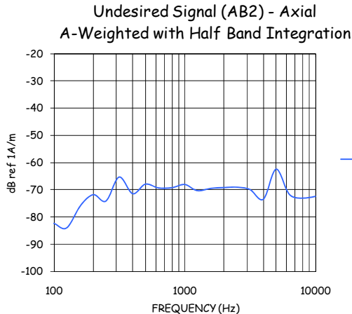
Figure 9-4-1: 900 MHz Undesired Signal (2:6).
