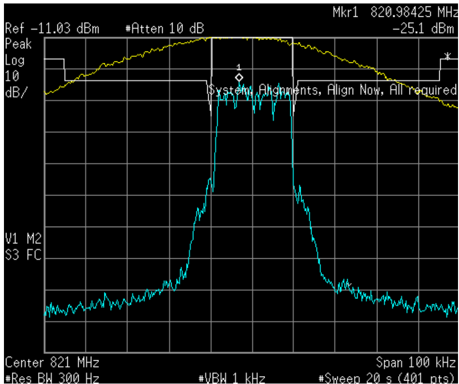
Figure 6a.2.1-6. iDEN 800 MHz Band, Quad-16QAM, Minimum Power, Emission Mask G
