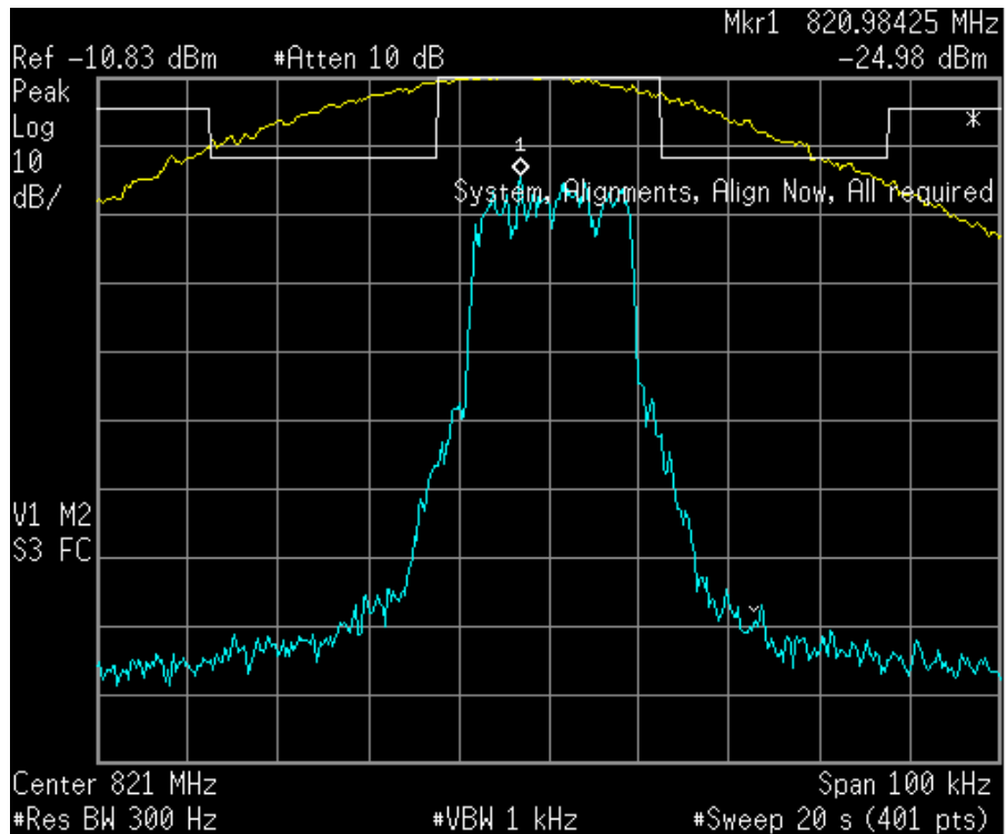
Figure 6a.2.1-8. iDEN 800 MHz Band, Quad-16QAM, Minimum Power, EA Emission Mask
