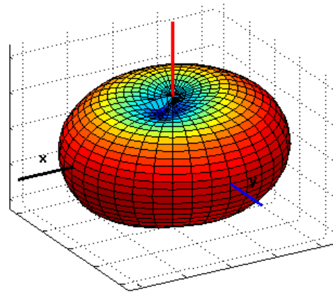
Figure 6a.6-2 Antenna pattern in the 800 MHz SMR frequency band (Flip Closed)
