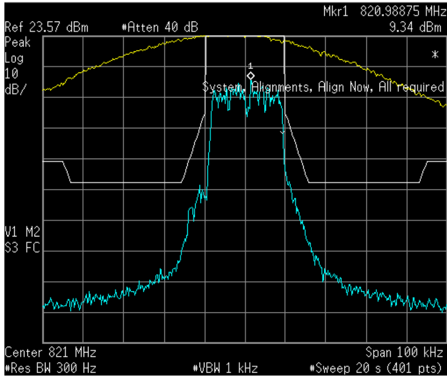
Figure 6a.2.1-9. iDEN 800 MHz Band, Quad-64QAM, Maximum Power, Emission Mask G
