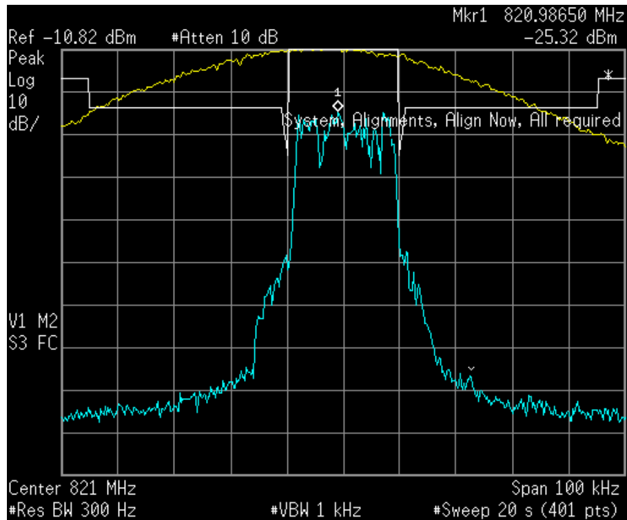
Figure 6a.2.1-10. iDEN 800 MHz Band, Quad-64QAM, Minimum Power, Emission Mask G
