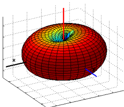
Figure 6a.6-5 Antenna pattern in the 900 MHz NBPCS frequency band (Flip Open).
