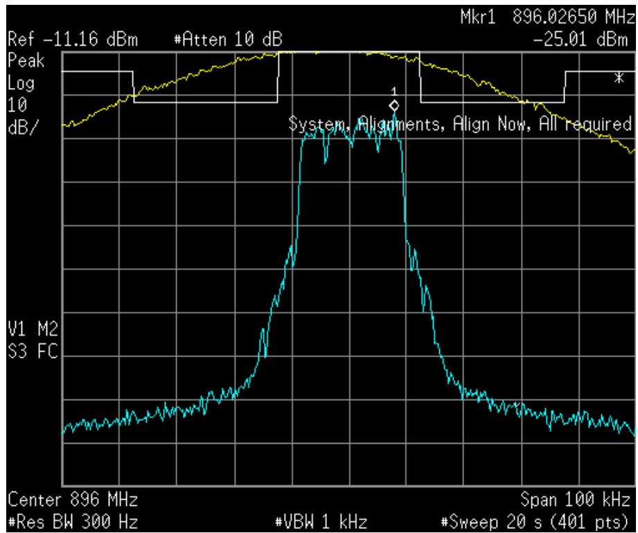
Figure 6a.2.2-8. iDEN 900 MHz Band, Quad-16QAM, Minimum Power, EA Emission Mask
