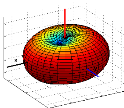
Figure 6a.6-6 Antenna pattern in the 900 MHz NBPCS frequency band (Flip Closed).
