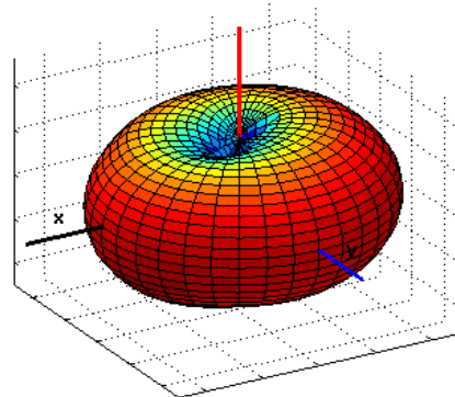
Figure 6a.6-4 Antenna pattern in the 900 MHz SMR frequency band (Flip Closed)
