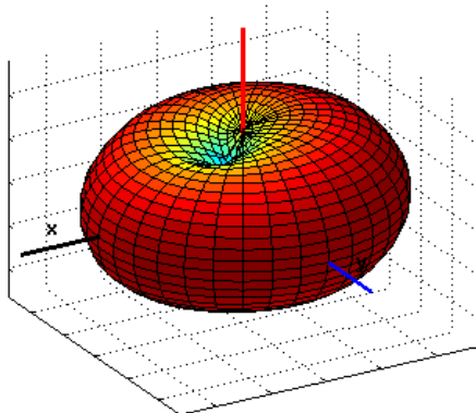
Figure 6a.6-3 Antenna pattern in the 900 MHz SMR frequency band (Flip Open).
