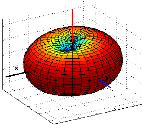
Figure 6a.6-1 Antenna pattern in the 800 MHz SMR frequency band (Flip Open).
