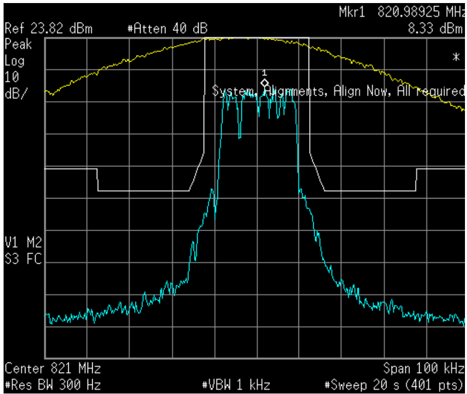
Figure 6a.2.1-11. iDEN 800 MHz Band, Quad-64QAM, Maximum Power, EA Emission Mask
