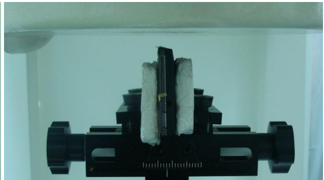
Left Side of the DUT with Phantom 1 cm Gap
