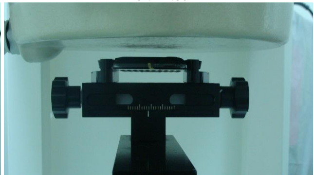
Back of the DUT with Phantom 1 cm Gap (DUT without Earphone)
