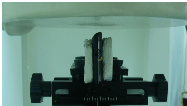
Right Side of the DUT with Phantom 1 cm Gap
