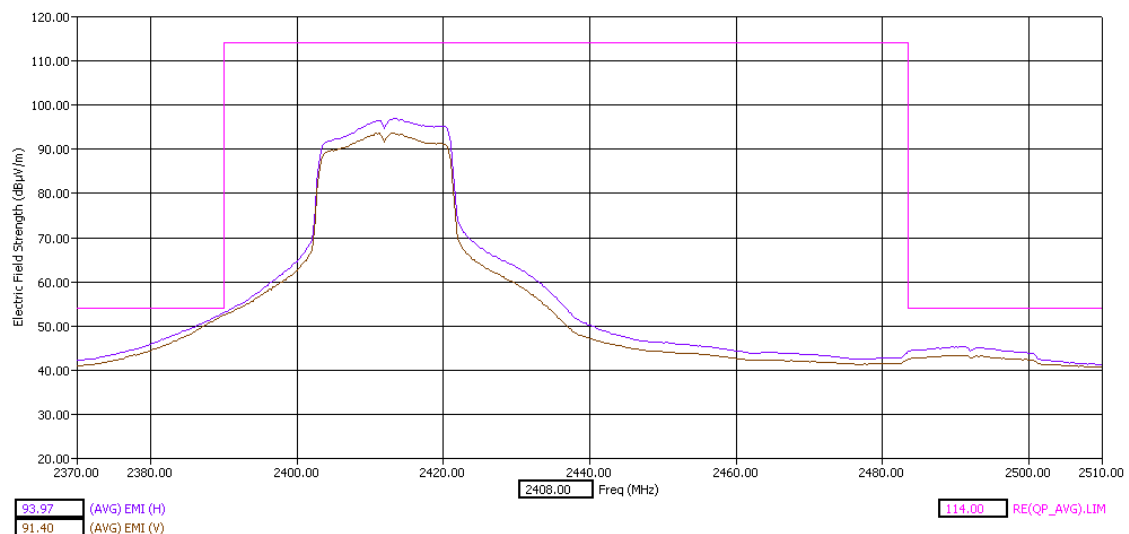
Low Band Edge Y Orientation AVG Detector
