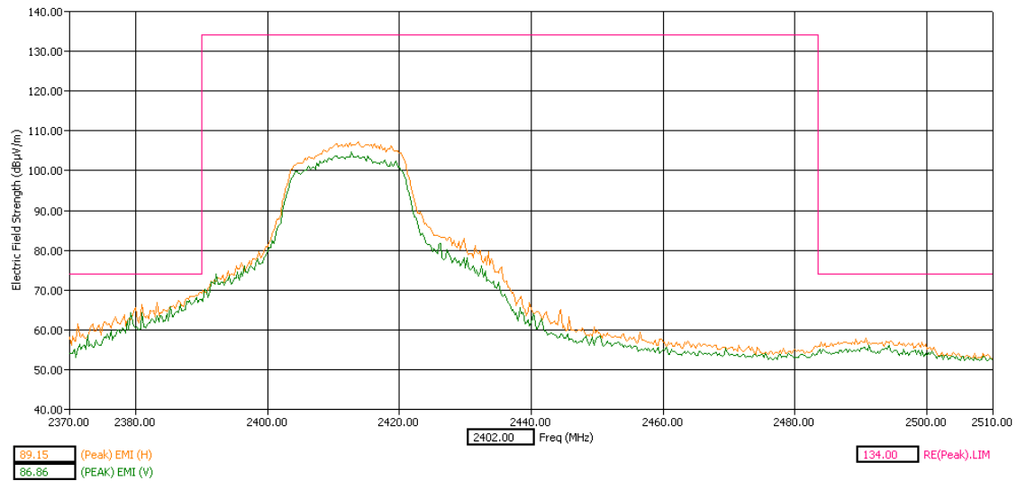
Low Band Edge Y Orientation Peak Detector
