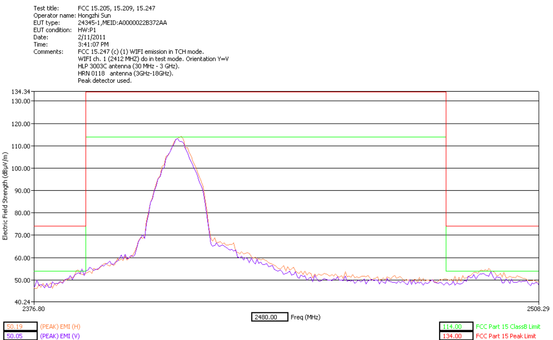
Low Band Edge Y Orientation Peak Detector
