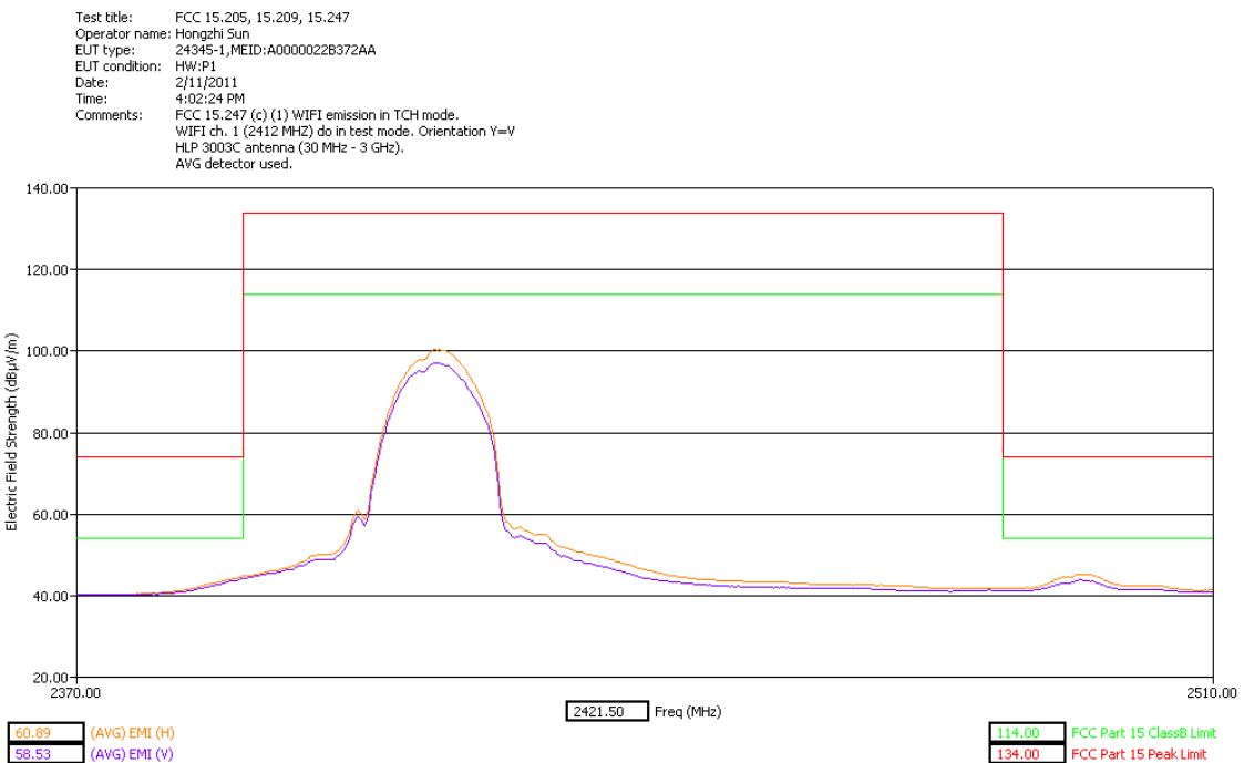
Low Band Edge Y Orientation AVG Detector
