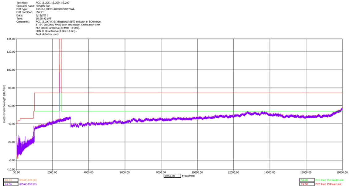
30 MHz – 18 GHz Low Channel Dual Polarization X
