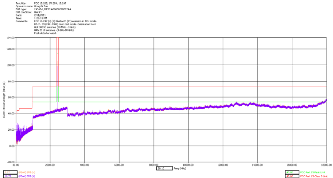
30 MHz – 18 GHz Middle Channel Dual Polarization X
