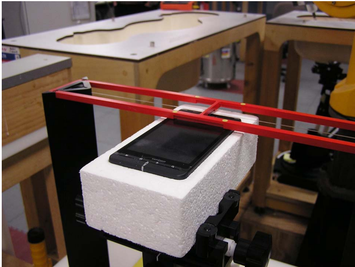
Figure 2. Positioning and Measurement for RF Emissions
