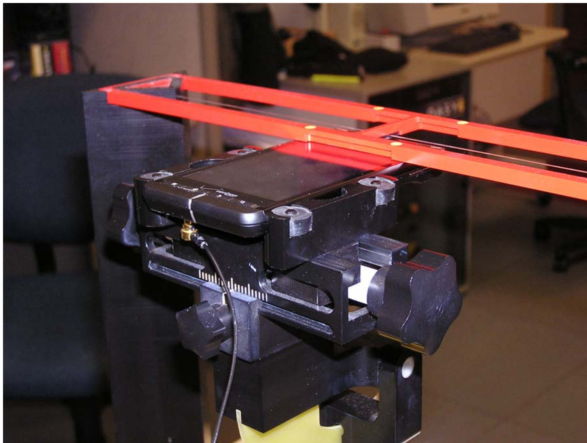
Figure 4. Positioning and Measurement for T-coil
