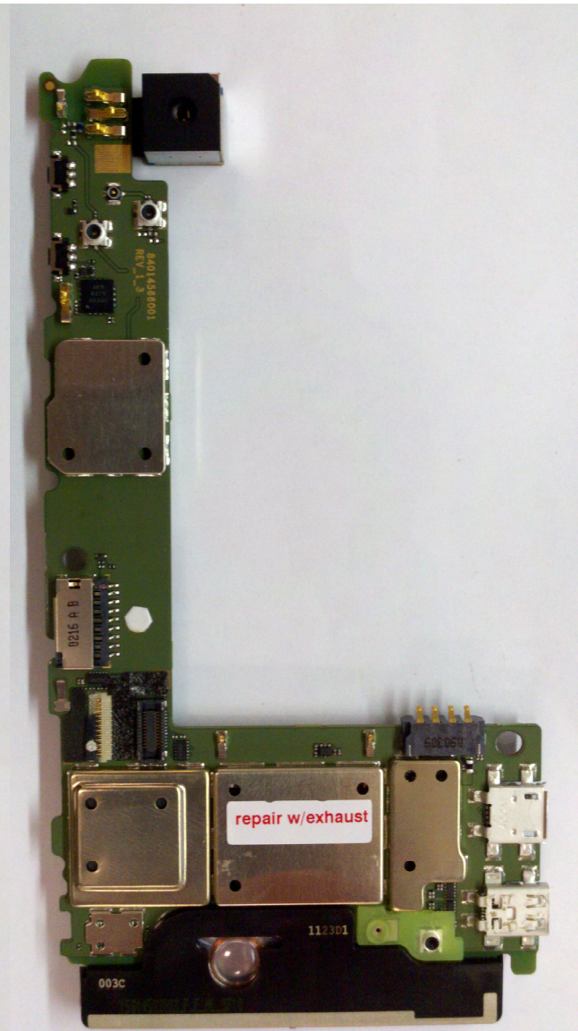
PCB - Rear
