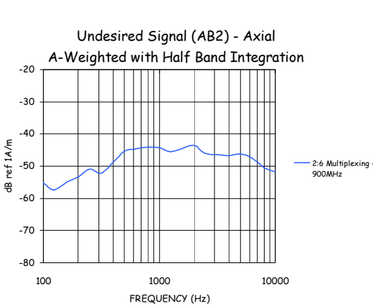
Figure 9-4-1: 900 MHz Undesired Signal (2:6)
