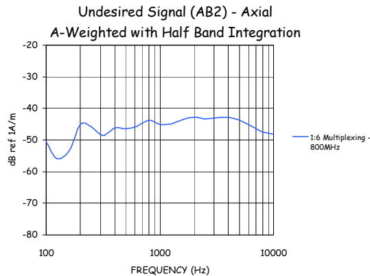
Figure 9-2-2: 800 MHz Undesired Signal (1:6)
