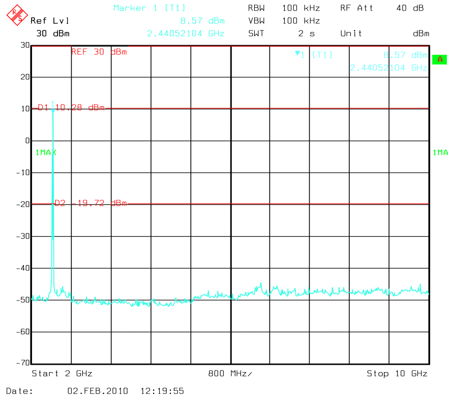
Figure 6c.5-6: Plot of Conducted Spurious Emissions, 2 – 10 GHz (11 Mbps data rate, Ch 6).
