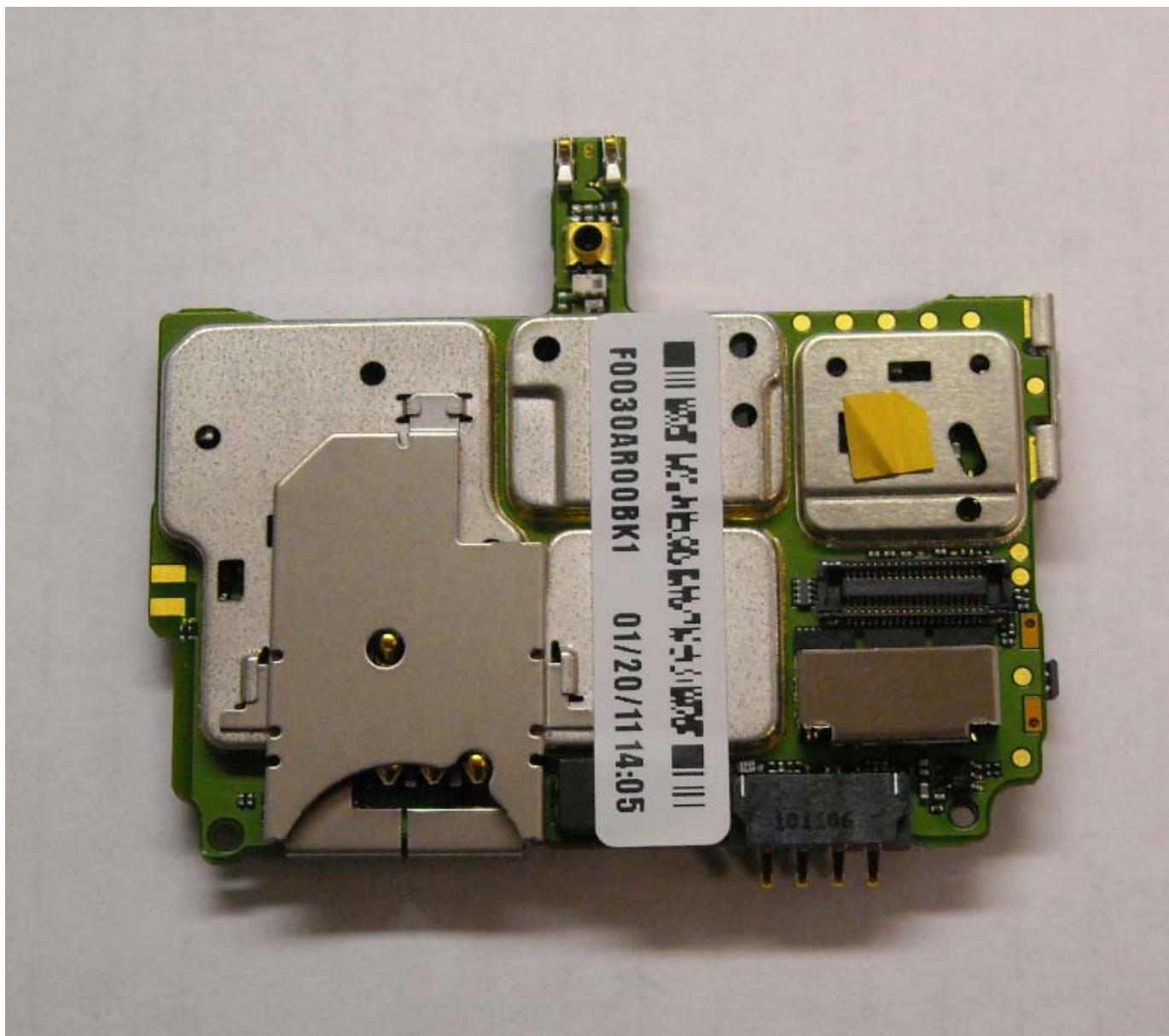
Photograph 9-3: Rear of Main PC Board, Shields in Place.
