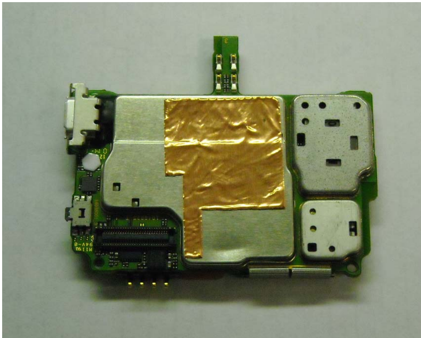
Photograph 9-1: Front Side of Main PC Board, Shields in Place.
