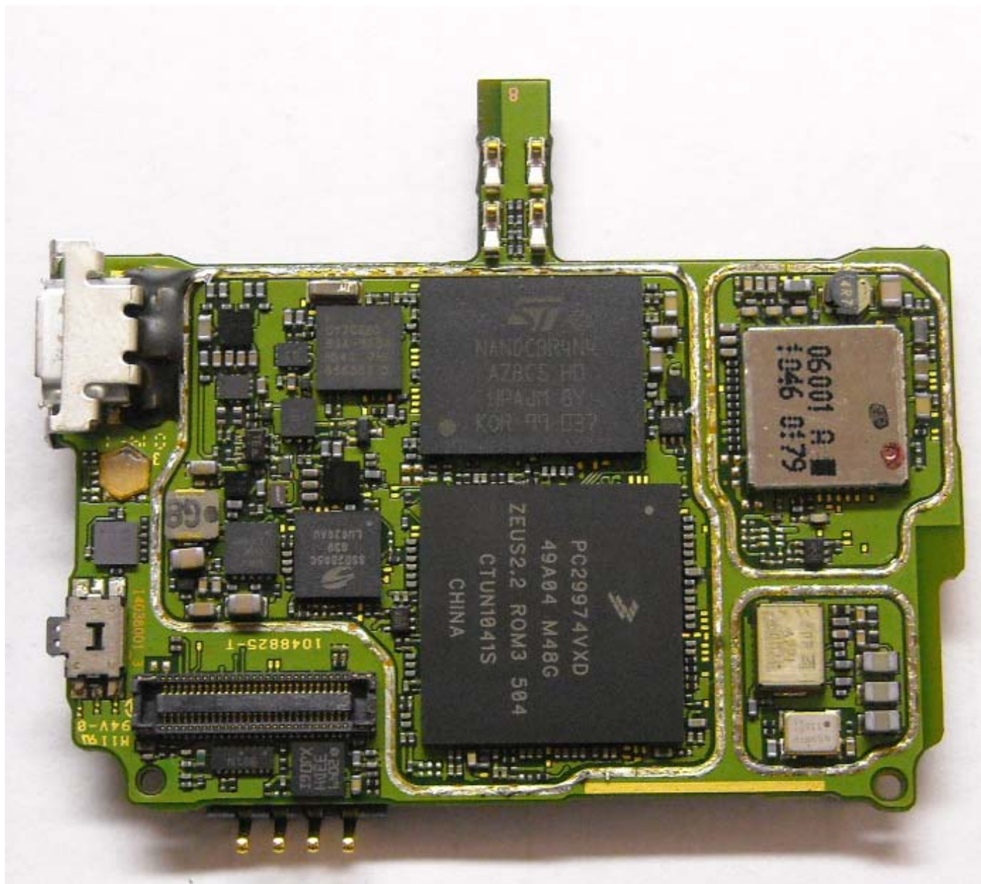
Photograph 9-2: Front of Main PC Board, Shields Removed.
