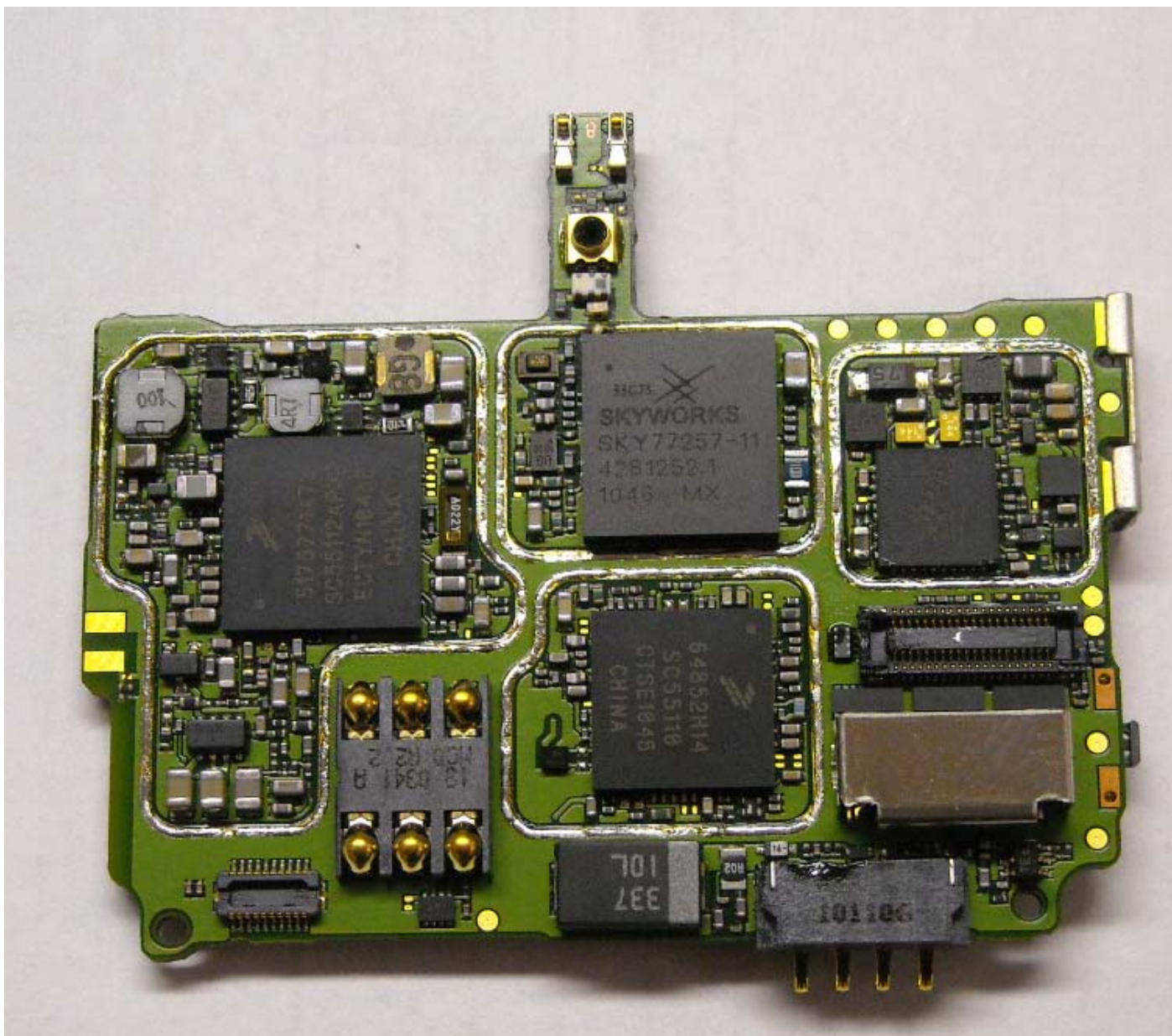
Photograph 9-4: Rear of Main PC Board, Shields Removed.
