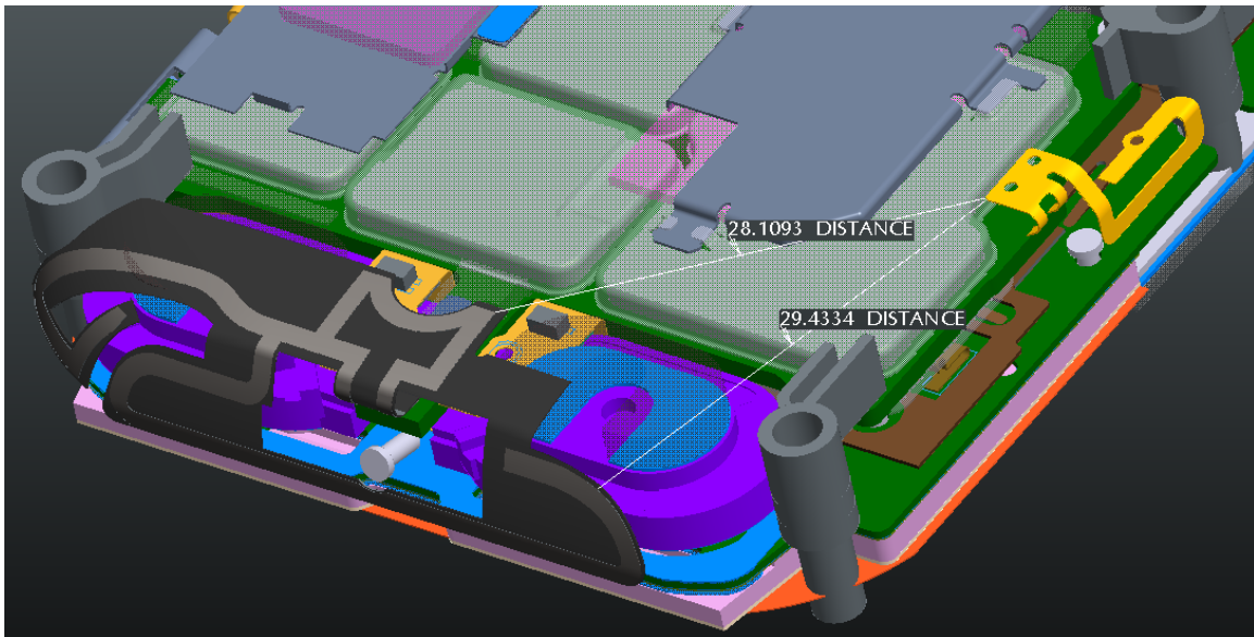
Figure 2: Antenna Separation Distances
